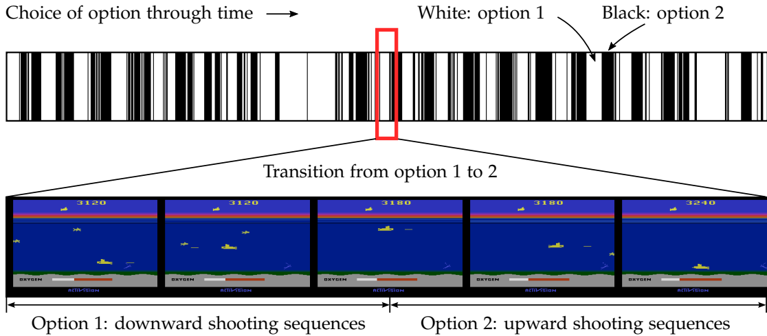
FIGURE 5.8 – Up/down specialization in the solution found by option-critic when learning with 2 options in Seaquest. The top bar shows a trajectory in the game, with “white” representing a segment during which option 1 was active and “black” for option 2.
