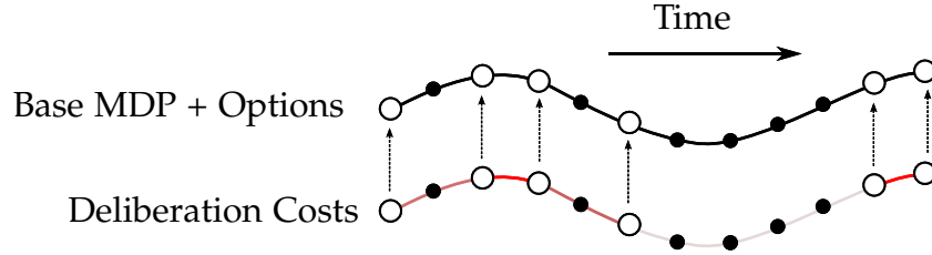
FIGURE 5.1 – The switching cost is incurred upon entering SMDP decision points, represented by open circles. The average decision cost per primitive step (filled circle) is represented by the intensity of the subtrajectory.
