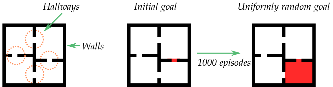
FIGURE 5.3 – Continuing transfer learning experiment in the four-rooms domain. After 1000 episodes, a new goal location is chosen randomly while continuing learning.
