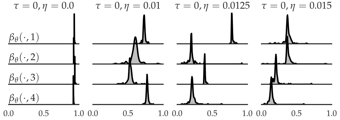
FIGURE 5.6 – Effect of regularization on the termination conditions parameterized with a bias term. Each graph is a kernel density plot over the termination probabilities \beta_\theta(\cdot, o) for each option, at all states. The vertical axis spans the options while the horizontal one is over different regularization coefficients.
