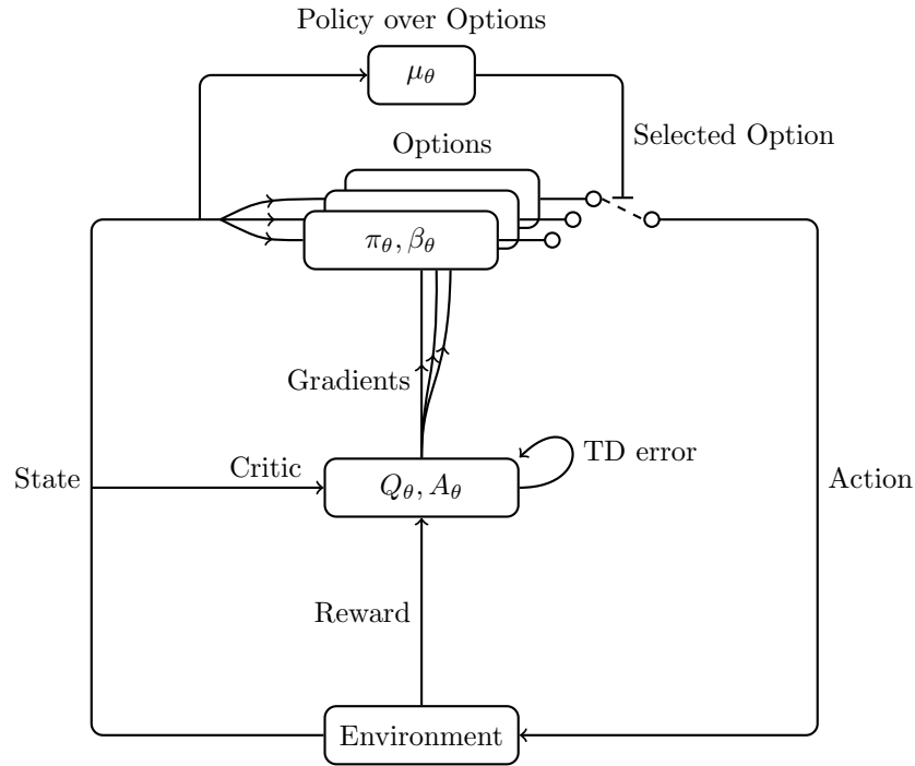
FIGURE 5.2 – Option-critic is an actor-critic architecture for learning options end-to-end. The actor contains a set of options parameterized by \theta and a policy over them \mu_\theta that are updated based on the value predictions made by a critic .
