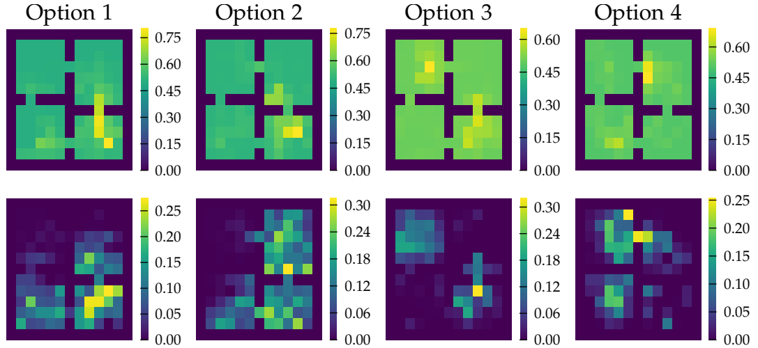
FIGURE 5.5 – Learned options after 2000 episodes. Top row: Termination probabilities for every options ie. \beta_{\theta}(\cdot, o) Bottom row: option policy weight corresponding to the preferred action (argmax) at every state
