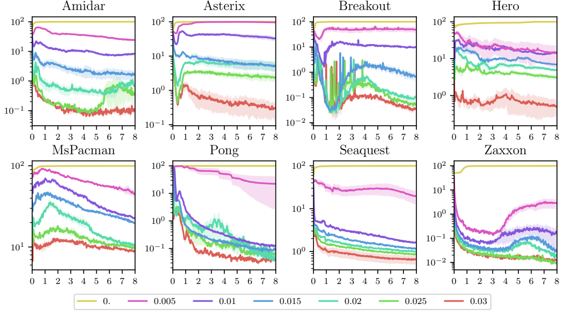
FIGURE 5.9 – Evolution of the empirical termination frequencies for different values of the regularization coefficient during learning (log scale). Without regularization, the options terminate after only one step. Larger values of the regularization coefficient result in more commitment during option execution.
