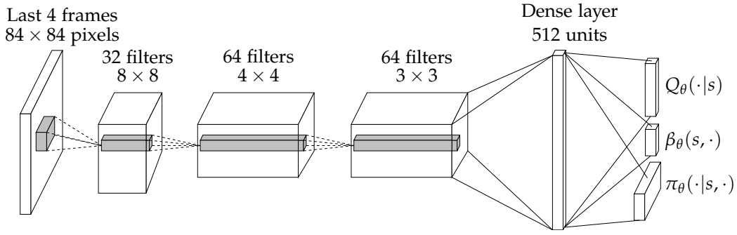
FIGURE 5.7 – Network architecture for DQN-OC. All the layers up to the penultimate one are the same as in the DQN architecture of Mnih et al. (2015).
