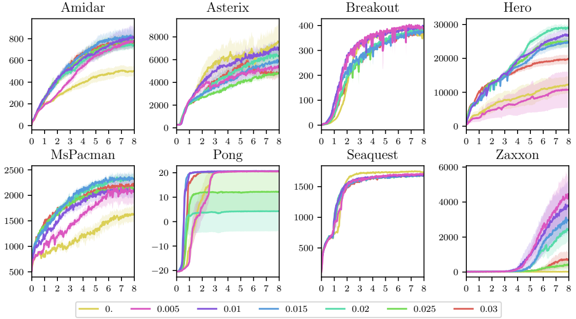
FIGURE 5.10 – Learning curves for A2OC averaged over 5 runs for different values of the regularization coefficient: intermediate values work best but also depend on environmental properties per game.
