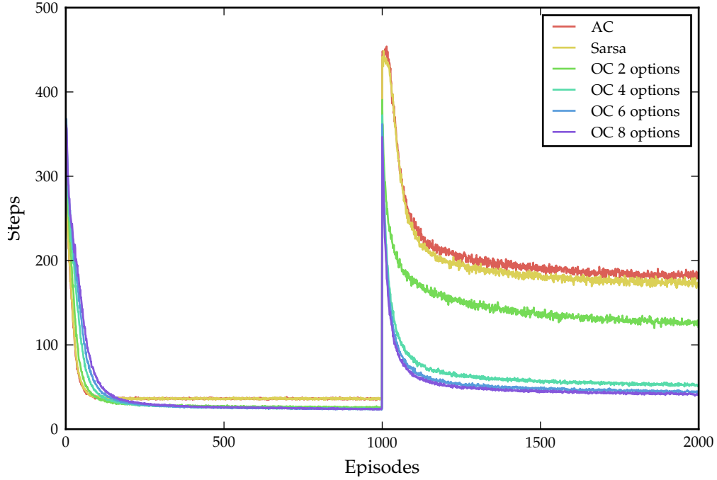
FIGURE 5.4 – Learning in the four-rooms domain: steps per episode (lower is better), averaged over 5000 runs. After 1000 episodes, the goal is moved randomly to a new location. “AC” stands for actor-critic, and “OC” for option-critic.
