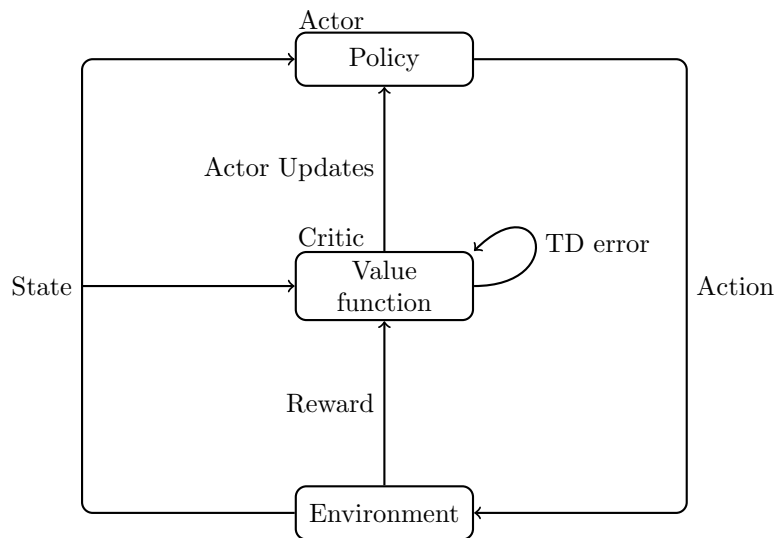
FIGURE 2.1 – The Actor-Critic Architecture
