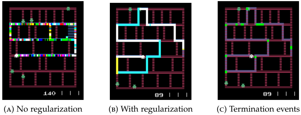
FIGURE 5.11 – Effect of the switching cost regularizer with \tau = \gamma in the game Amidar. Each segment of color is a subtrajectory under a given option. The last panel (c) shows the location of the termination events along the trajectory shown in (b).
