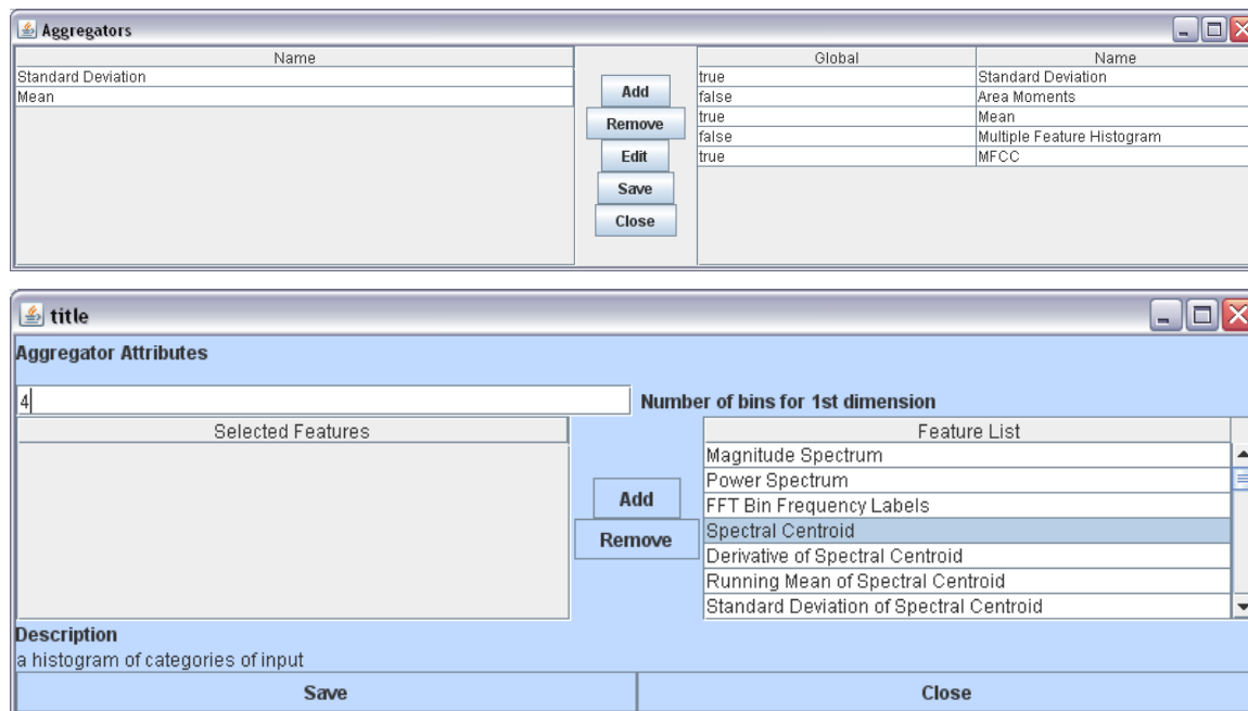
Figure 3.11: jAudio windows allowing aggregators to be selected (top) and configured (bottom).
