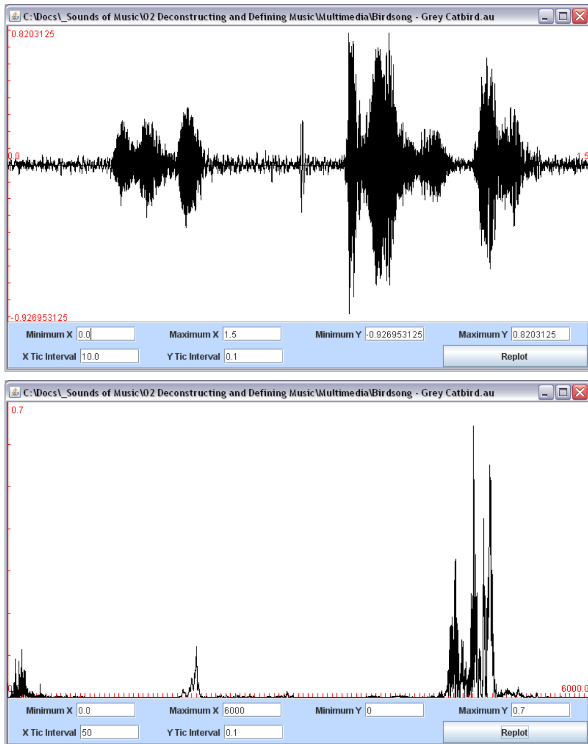
Figure 3.13: jAudio windows for displaying waveforms (top) and power spectra (bottom) for all or parts of audio files.
