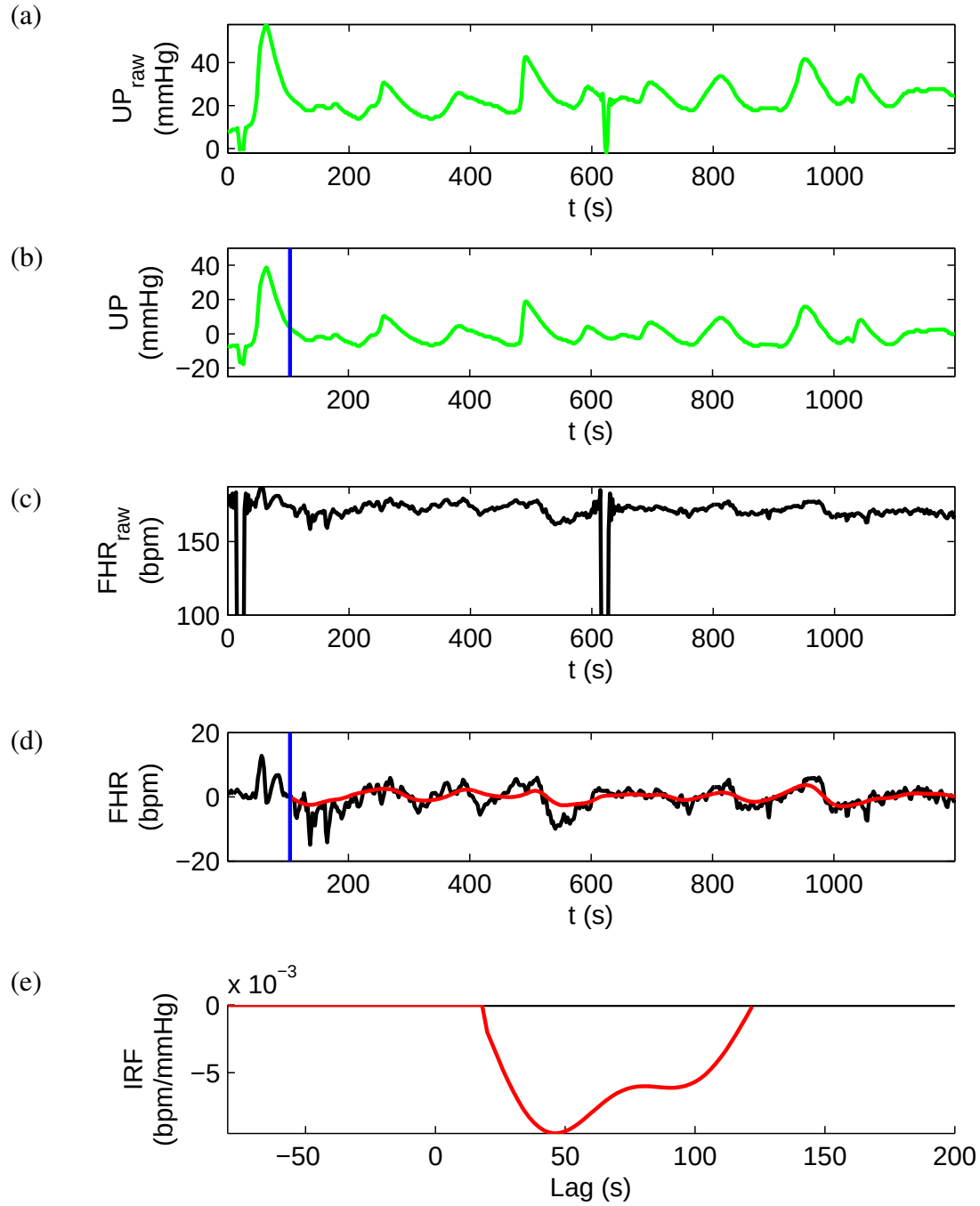
Fig. 2. System identification modelling results for an typical epoch of a pathological case. (a) raw input UP (b) pre-processed UP (c) raw output FHR (d) preprocessed (black) and predicted (red) output FHR (e) final IRF. The IRF delay d was 20 s, the gain G was -0.32 bpm/mmHg and the VAF of the model was 44.0.
