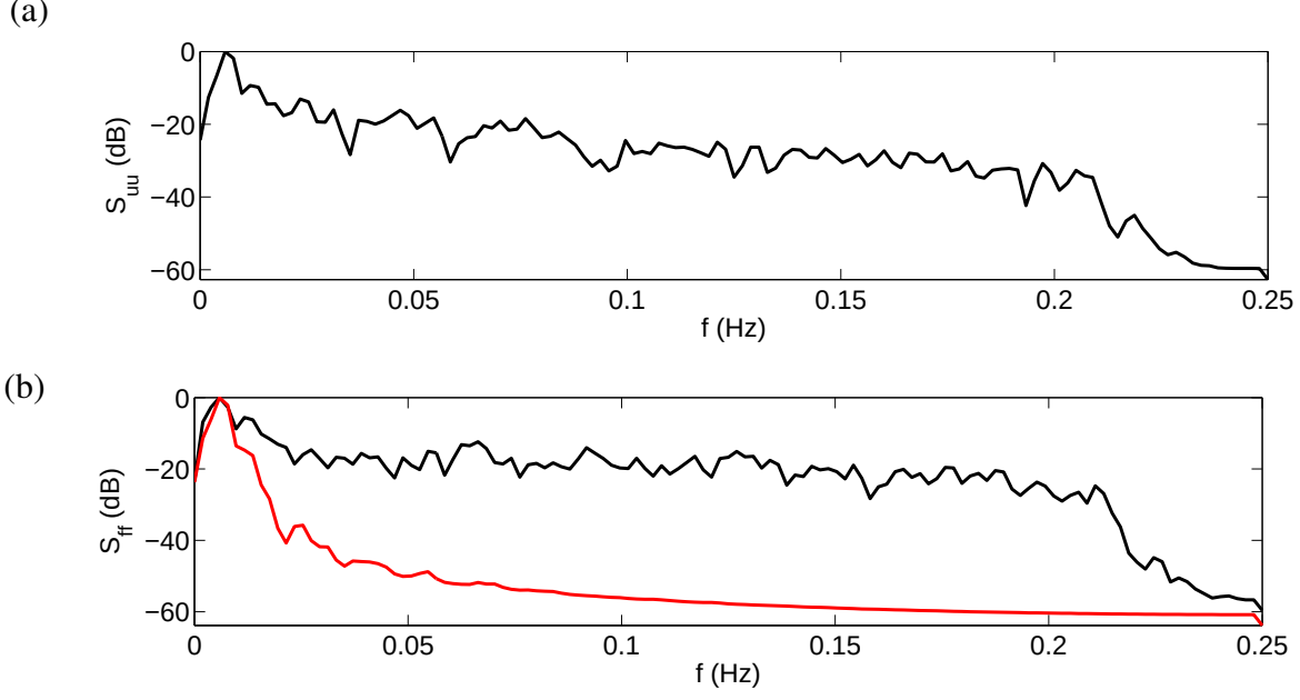
Fig. 7. Frequency analysis for an example epoch for a normal case. (a) input UP spectrum S_{uu} (b) preprocessed (black) and predicted (red) output FHR spectra S_{ff} and S_{\hat{f}\hat{f}} .
