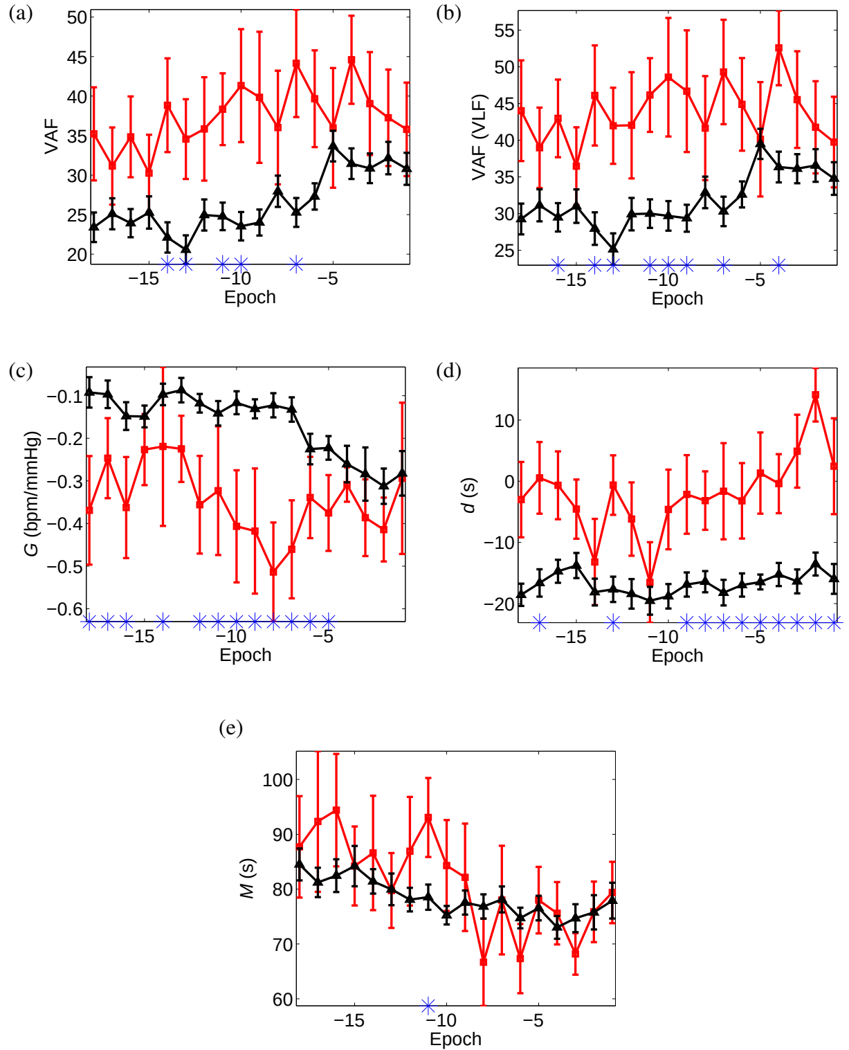
Fig. 10. Time progression of model parameters in the last three hours of labour and delivery. The mean and standard error for (a) VAF, (b) VAF VLF (c) gain G , (d) delay d and (e) memory M are plotted by epoch for normal (black triangles) and pathological (red squares) cases. For each parameter, epochs where hypothesis tests indicated significant differences between classes ( p < 0.05 ) are displayed by asterisks (*).
