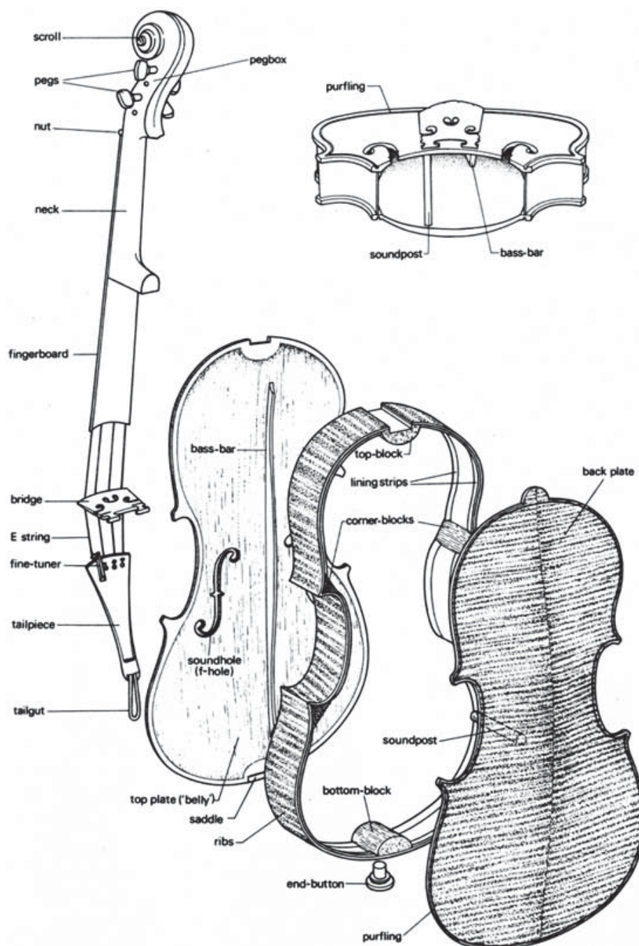
Figure 2.2: An exploded view of the violin. From Johannsson (2015).
