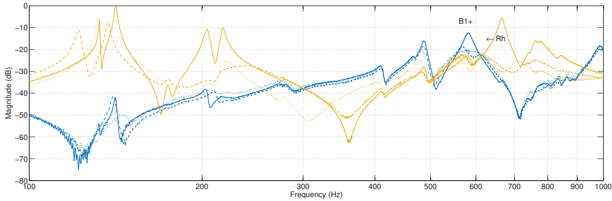
Figure 4.11: FRFs from the bridge (blue) overlaid onto those from IP 2 of the tailpiece (gold) demonstrate the coupling between the B1+ and Rh modes after a 5.5 g mass was attached at position 1 (dashed line) and position 2 (dotted line), compared to having the mass off (solid line). The arrow indicates the downward shift of the Rh mode.
