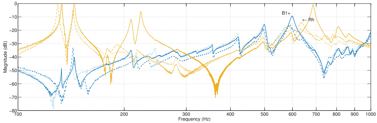
Figure 4.8: FRFs from the bridge (blue) overlaid onto those from IP 2 of the tailpiece (gold) demonstrate the coupling between the B1+ and Rh modes after a 2.5 g mass was attached at position 1 (dashed line) and position 2 (dotted line), compared to having the mass off (solid line). The arrow indicates the downward shift of the Rh mode.
