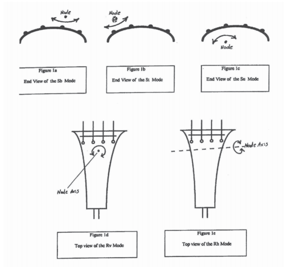
Figure 2.4: Tailpiece modes as depicted by Stough (1996), demonstrating the three “swing” modes (top) and the two rotation modes (bottom).
