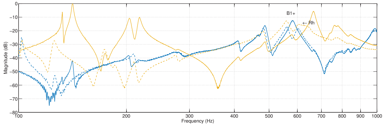
Figure 4.17: FRFs from the bridge (blue) overlaid onto those from IP 2 of the tailpiece (gold) demonstrate the coupling between the B1+ and Rh modes of a violin outfitted with one fine tuner (solid) versus four (dashed). The arrow indicates the downward shift of the Rh mode.
