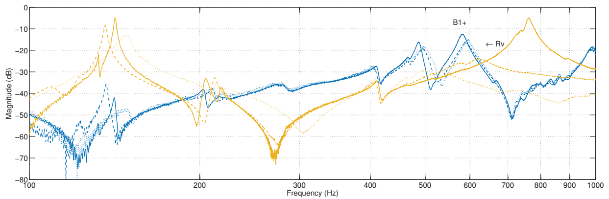
Figure 4.14: FRFs from the bridge (blue) overlaid onto those from IP 2 of the tailpiece (gold) demonstrate a possible coupling between the B1\pm and Rv modes after a 16.0 g mass was attached at position 1 (dashed line) and position 2 (dotted line), compared to having the mass off (solid line). The arrow indicates the downward shift of the Rv mode.
