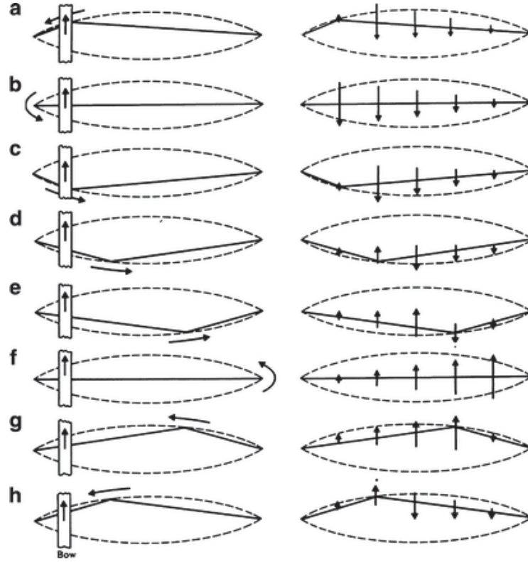
Figure 2.3: A time-lapse representation of Helmholtz motion. (Left) The bend in the string (the “Helmholtz corner”) traces out a curved path as it travels along the string; (right) the associated velocities of the string. From Rossing et al. (2002).
