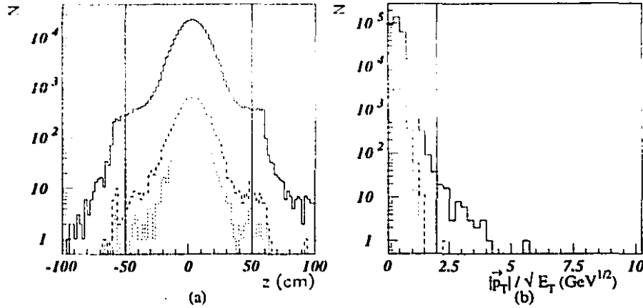
Figure 3.6: The distribution of the z -position of the reconstructed vertex is shown in (a). The distribution of the relative missing transverse momentum in the calorimeter, |p_T|/\sqrt{E_T} , is shown in (b). The solid line shows a loose sample of dijet events. The dashed line shows the sample of dijet events which will be used in this analysis and the dotted line shows a clean sample of photoproduction events where the scattered e^+ is measured in the e^+ LUMI detector.
