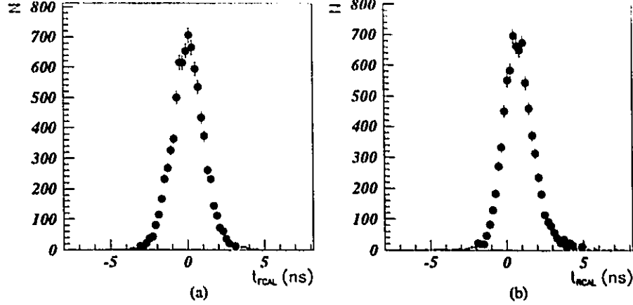
Figure 3.2: The distribution of the average time of FCAL energy deposits is shown in (a) and the distribution of the average time of RCAL energy deposits is shown in (b).
