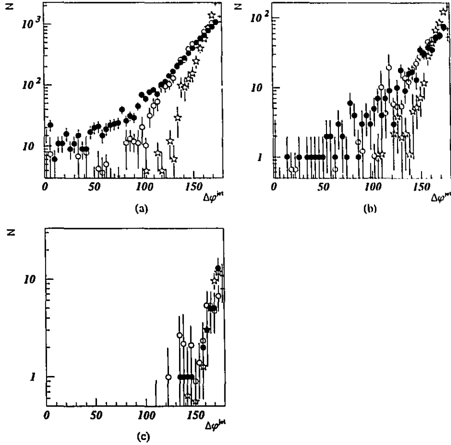
Figure C.1: Relative azimuth of the two highest E_T^{jet} jets for the inclusive sample is shown in (a). \Delta\phi^{jet} for the subsample with \Delta\eta > 3.5 is shown in (b) and (c) shows the gap candidate events with \Delta\eta > 3.5 . The data are shown by the black dots. The open circles represent the PYTHIA sample which includes no colour singlet exchange processes (the non-singlet sample). The stars represent the PYTHIA sample which contains only electroweak quark quark scattering (the singlet sample).
