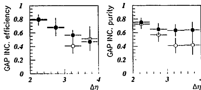
Figure 5.10: The gap incremental bin-efficiency is shown on the left and the gap incremental bin-purity is shown in the right. The non-singlet PYTHIA sample is shown by the open circles and the mixed PYTHIA sample is shown by the black dots.
