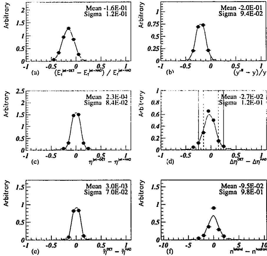
Figure 4.18: Resolutions of the kinematic variables, according to the PYTHIA sample which contains 10% of colour singlet exchange processes (the mixed sample). The resolution of E_T^{jet} is shown in (a), the resolution of y is shown in (b), the resolution of \eta^{jet} is shown in (c), the resolution of \Delta\eta is shown in (d), the resolution of \eta is shown in (e) and the multiplicity resolution is shown in (f). The dashed (solid) vertical lines in (d) show the bin width chosen for the uncorrected (corrected) \Delta\eta distributions.
