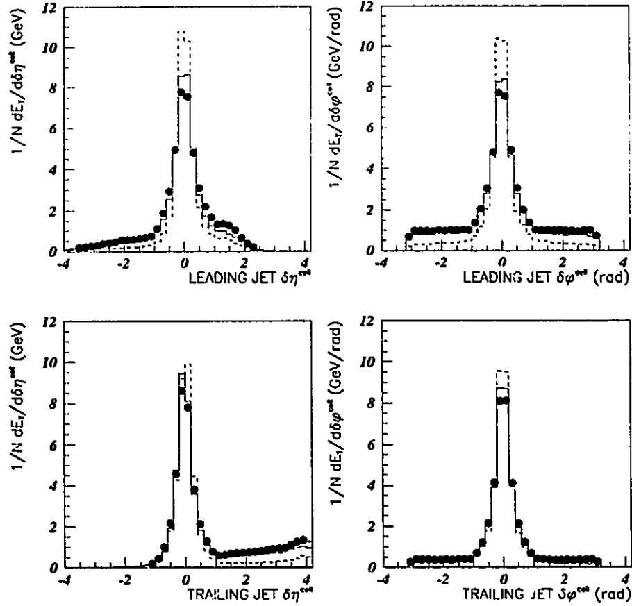
Figure 4.7: Jet profiles for the leading and trailing jets. The data are shown as black dots. The prediction of the PYTHIA sample with no colour singlet exchange (the non-singlet sample) is shown by the solid line. The prediction by the PYTHIA sample with only electroweak quark-quark scattering (the singlet sample) is shown by the dashed line.
