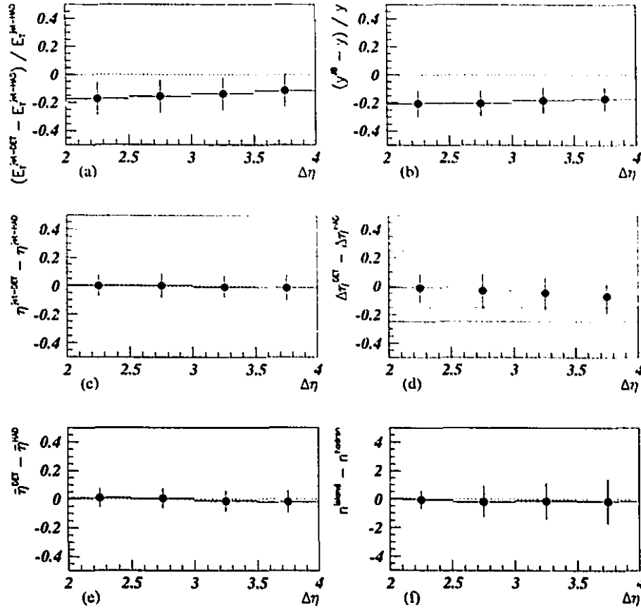
Figure 5.13: Resolution versus \Delta\eta . The black dot shows the shift and the error bars show the width.
