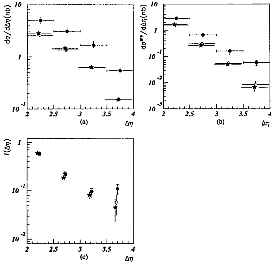
Figure 6.4: The data (corrected for detector effects) are shown as black dots where the inner error bar shows the statistical error and the outer error bar shows the systematic uncertainty added in quadrature. The HERWIG predictions including multiple interactions are shown as solid stars and the open crosses show the HERWIG predictions without multiple interactions.
