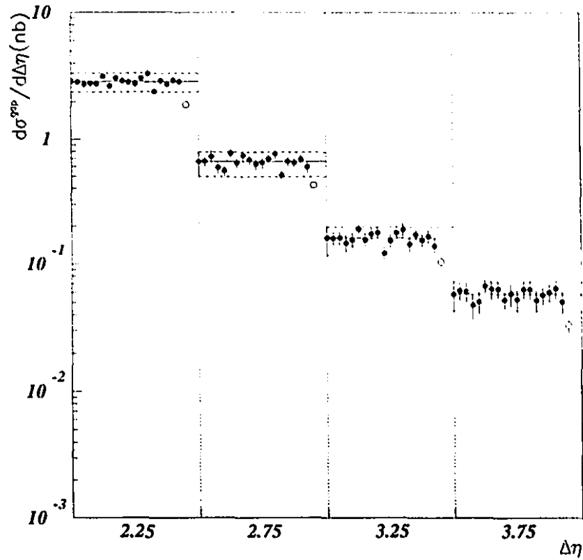
Figure 5.15: The gap cross section computed in seventeen different ways (see text) is shown by the black dots and the white dots show the distribution before the detector corrections for comparison.
