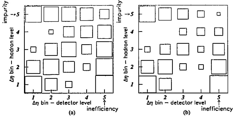
Figure D.2: Cause versus effect according to the mixed Monte Carlo sample. The correlation between the hadron-level and detector-level \Delta\eta values is shown by the intersection of the first four rows and columns. The fifth column shows the hadron-level events which were not found as detector-level events. The fifth row shows the detector-level events which have not arisen from hadron-level events. The inclusive sample of events is shown in (a) and the subsample of events which are gap candidates is shown in (b).
