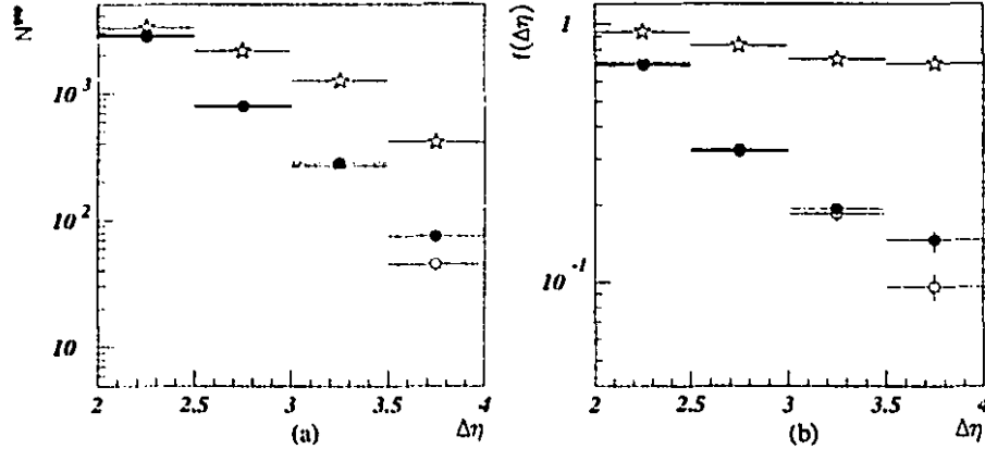
Figure 5.6: The \Delta\eta distribution for gap events where a gap is defined as \leq 1 track with E_T^{track} > 200 MeV is shown in (a). The corresponding gap-fraction is shown in (b). The data are shown as black dots. The prediction by the PYTHIA non-singlet sample is shown by open circles and the prediction by the PYTHIA singlet sample is shown by stars.
