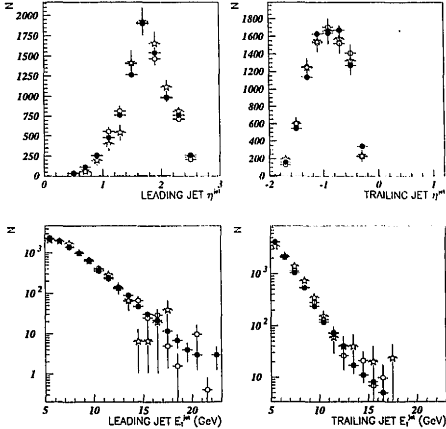
Figure 4.10: The distributions of \eta^{jet} and E_T^{jet} for the leading and trailing jets. The ZEUS data are shown by black dots. The prediction by the PYTHIA sample with no colour singlet exchange events (the non-singlet sample) is shown by the open circles and the prediction by the PYTHIA sample with only electroweak quark-quark scattering (the singlet sample) is shown by the stars.
