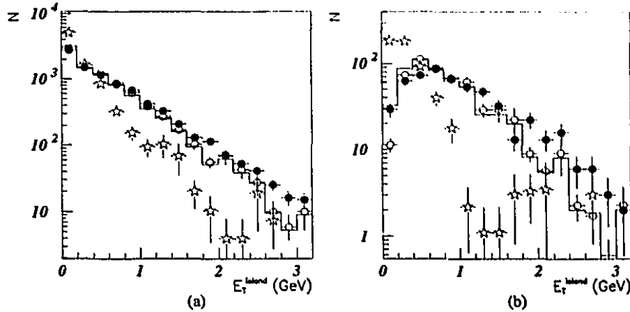
Figure 4.14: The E_T^{island} distribution of the maximum E_T^{island} island between the jets. The ZEUS data are shown by black dots. The prediction by the PYTHIA sample with no colour singlet exchange events (the non-singlet sample) is shown by the open circles and the prediction by the PYTHIA sample with only electroweak quark-quark scattering (the singlet sample) is shown by the stars. The prediction by the PYTHIA sample with 10% of electroweak exchange processes (the mixed sample) is shown by the solid line. In (a) the distribution is shown for all events and in (b) the distribution is shown just for the subsample with \Delta\eta > 3.5 .
