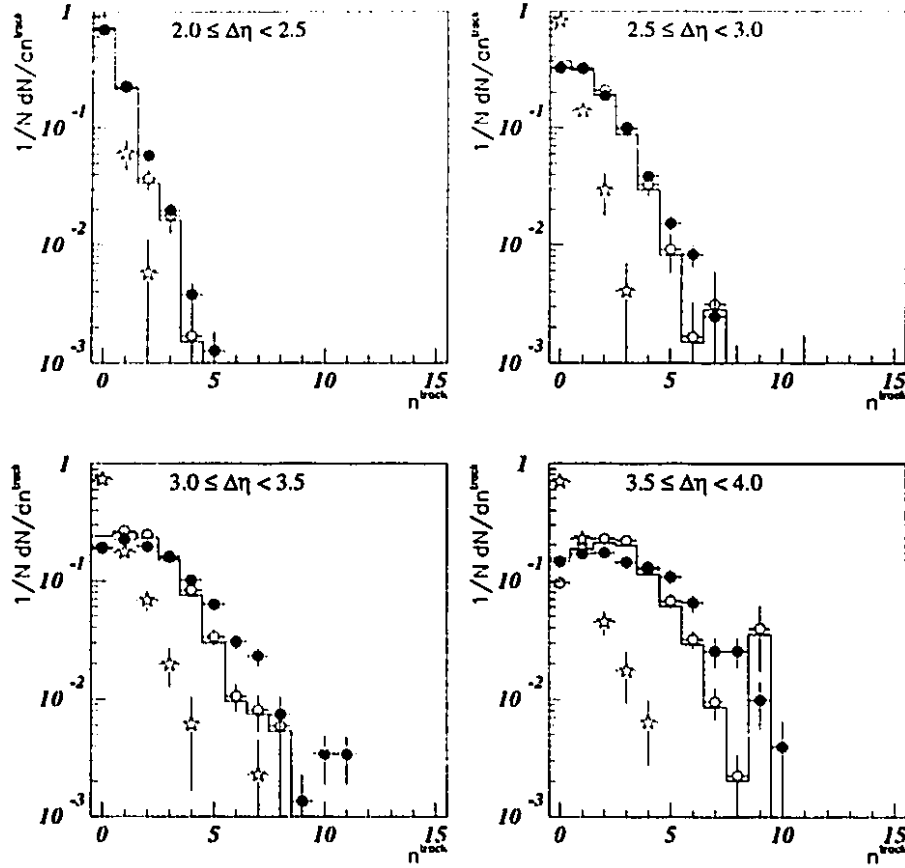
Figure 5.2: The charged multiplicity distributions in four bins of \Delta\eta . The data are shown as black dots. The prediction by the PYTHIA non-singlet sample is shown by open circles and the prediction by the PYTHIA singlet sample is shown by stars. The solid line shows the prediction of the PYTHIA mixed sample.
