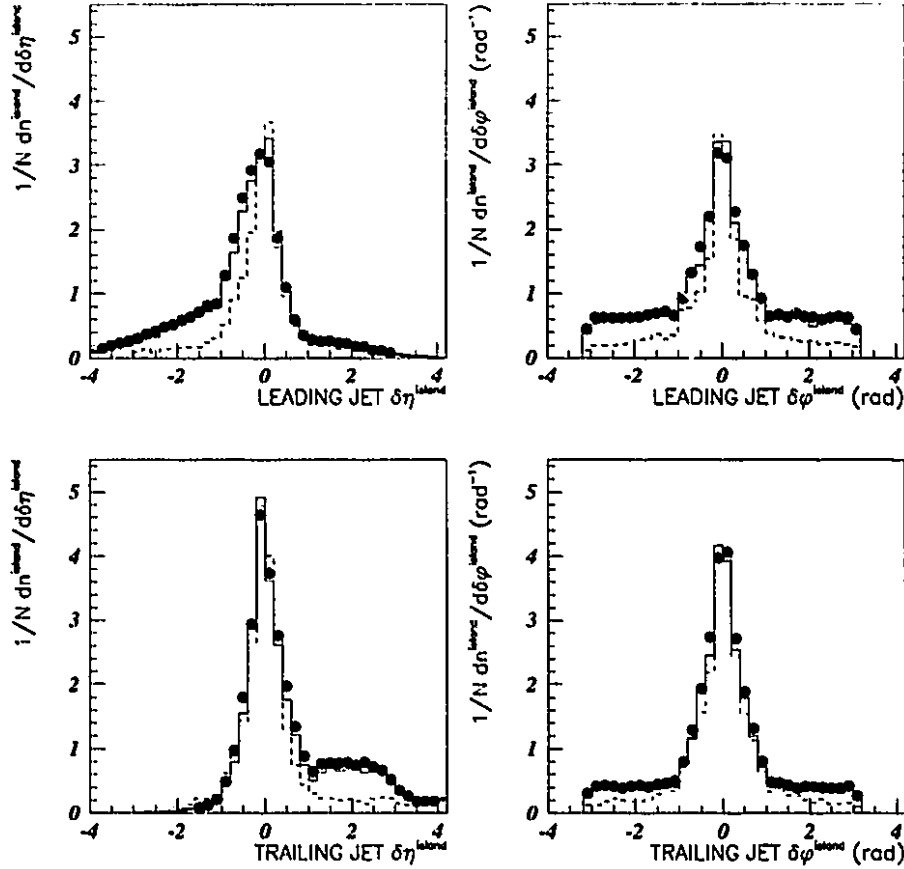
Figure 4.13: The distributions of \delta\eta^{island} and \delta\phi^{island} with respect to the centres of the leading and trailing jets. The data are shown as black dots. The prediction of the PYTHIA sample with no colour singlet exchange (the non-singlet sample) is shown by the solid line. The prediction by the PYTHIA sample with only electroweak quark-quark scattering (the singlet sample) is shown by the dashed line.
