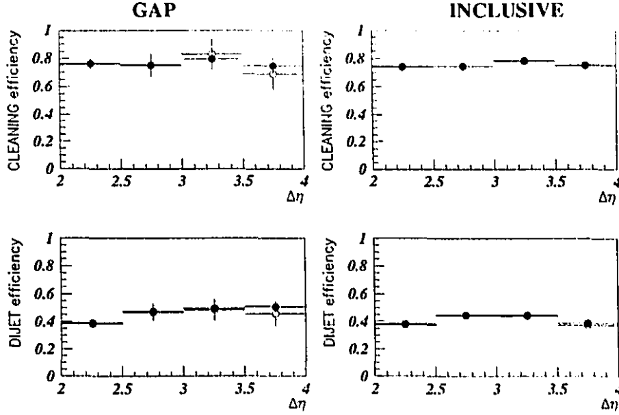
Figure 4.17: The first row shows the cumulative efficiency up to the offline cleaning criteria and the second row shows the cumulative efficiency up to the definition of the reconstructed jets. The efficiency for gap events is shown on the left and the efficiency for the inclusive sample is shown on the right. The non-singlet sample efficiencies are shown as open circles and the mixed sample efficiencies are shown as black dots.
