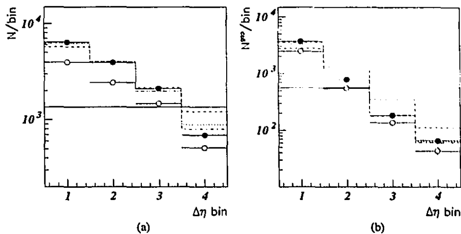
Figure D.5: Unfolding of the measured \Delta\eta distributions of the data using the mixed Monte Carlo sample inputs. The starting distribution is represented by the solid line and the dashed, dotted and dashed dotted lines represent the first, second and third iterations respectively. The final iteration is shown by the black dots. The open circles show the uncorrected distributions.
