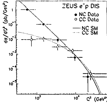
Figure 1.1: ZEUS measurement of d\sigma/dQ^2 for neutral current interactions (black dots) and charged current interactions (open circles). The data are plotted at the average Q^2 of the events in each bin. The curves are the standard electroweak model cross sections.
