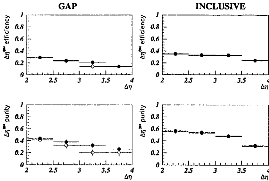
Figure 5.9: The bin-efficiencies are shown in the first row and the bin-purities are shown in the second row. The first column shows the subsample of events which are hadron-level gap events and the second column shows the inclusive sample of events. The non-singlet PYTHIA sample is shown by the open circles and the mixed PYTHIA sample is shown by the black dots.
