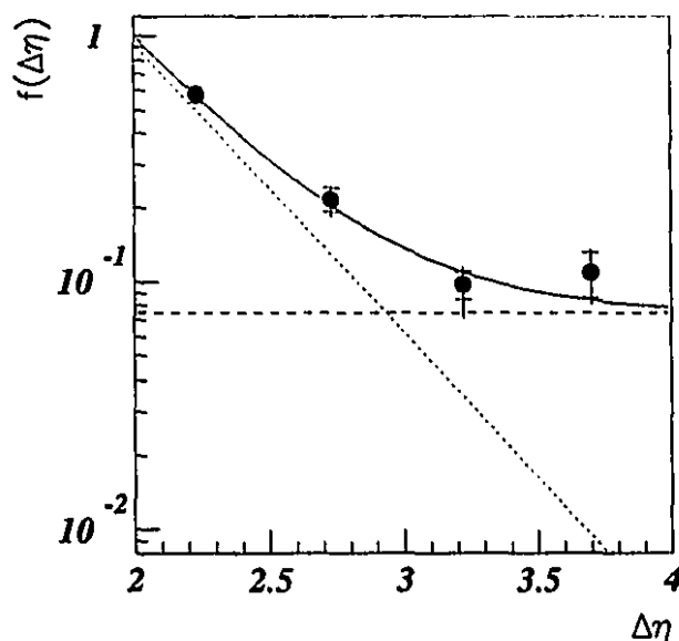
Figure 6.5: The gap-fraction, f(\Delta\eta) , with a fit to the expression, f = C(\alpha, \beta)e^{\alpha\Delta\eta} + \beta shown as the solid line. The dotted line shows the exponential term and the dashed line shows the constant term.
