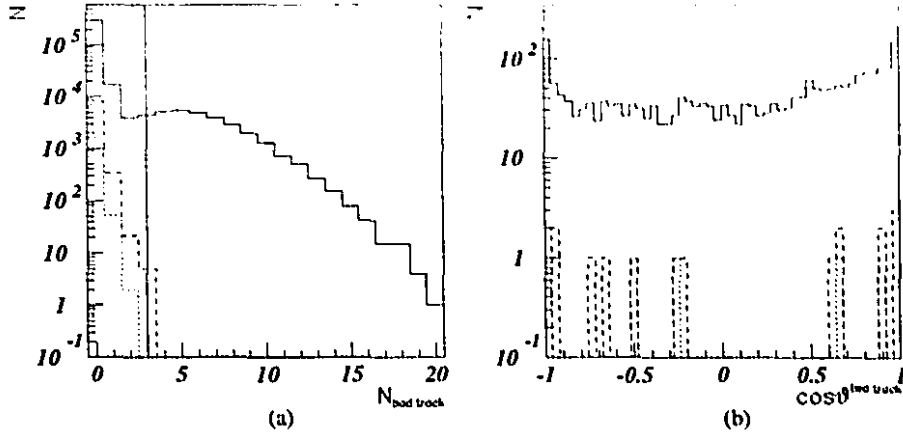
Figure 3.5: Tracking cuts to suppress beam-gas and cosmic contamination. The solid line shows a loose sample of dijet events. The dashed line shows the sample of dijet events which will be used in this analysis and the dotted line shows a clean sample of photoproduction events where the scattered e^+ is measured in the e^+ LUMI detector. The distribution of the number of tracks which point to a vertex in the rear is shown (a). The distribution of the opening angle between the two tracks for events which have only two tracks is shown in (b).
