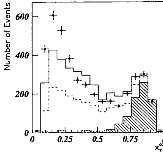
Figure 1.5: The ZEUS 1993 measurement of x_{\gamma}^{cal} . The black dots show uncorrected ZEUS data. The solid and dashed lines show the predictions of two different Monte Carlo simulation routines. The LO direct contribution to the distribution shown by the dashed line, is represented by the hashed histogram. The Monte Carlo curves have been normalized to fit the direct peak in the data.
