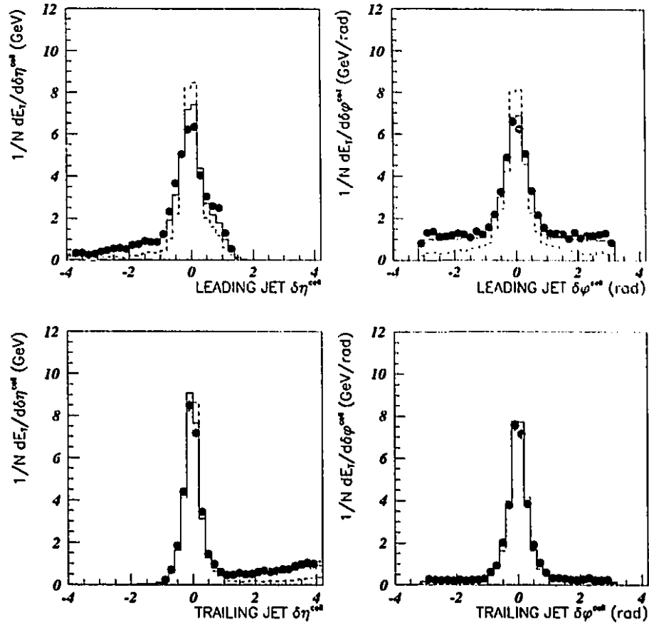
Figure 4.8: Jet profiles for the leading and trailing jets, for the subsample of events with \Delta\eta > 3.5 . The data are shown as black dots. The predictions of the PYTHIA singlet and non-singlet samples are shown by the solid and dashed lines respectively.
