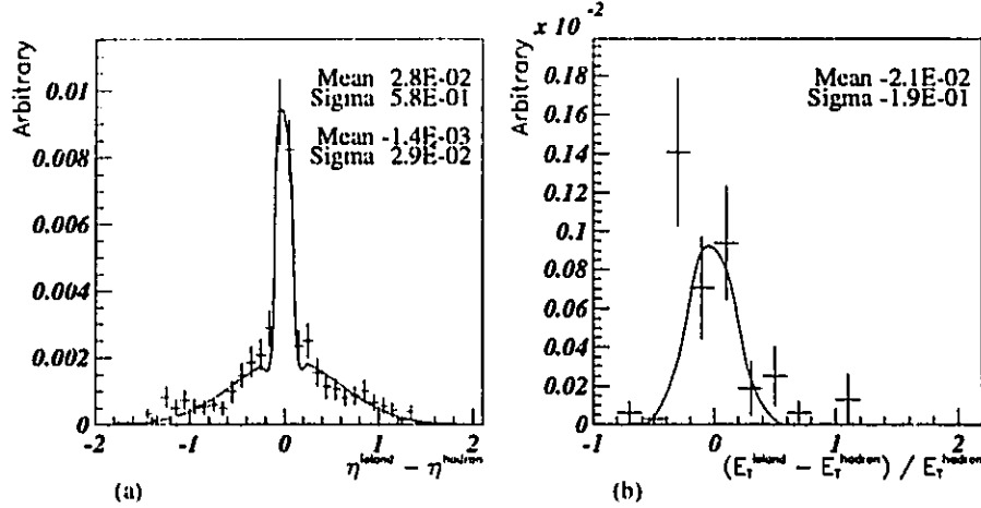
Figure 4.20: Resolution of the island angle and energy according to the mixed Monte Carlo sample for the subsample of events with \Delta\eta > 3.5 . The \eta^{\text{hadron}} resolution is shown in (a) and the E_T^{\text{hadron}} resolution is shown in (b).
