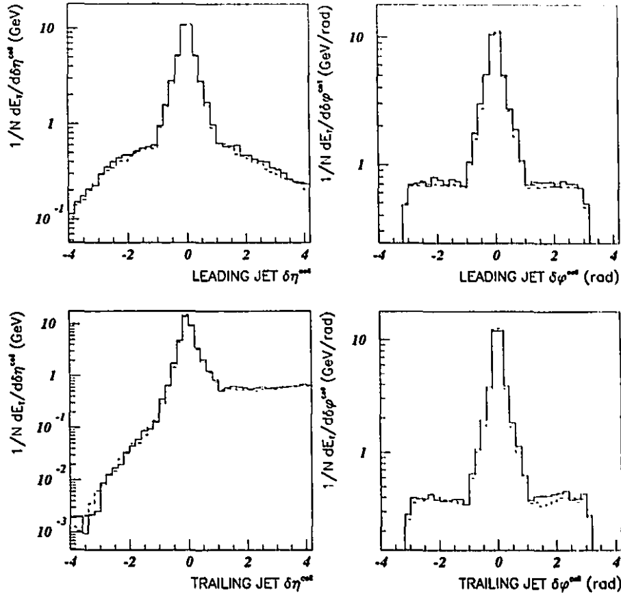
Figure 6.3: Hadron-level jet profiles are shown separately for the leading and trailing jets. The solid line shows the jet profiles of the non-singlet sample and the dashed line shows the jet profiles of the low \sigma_{PT} sample.
