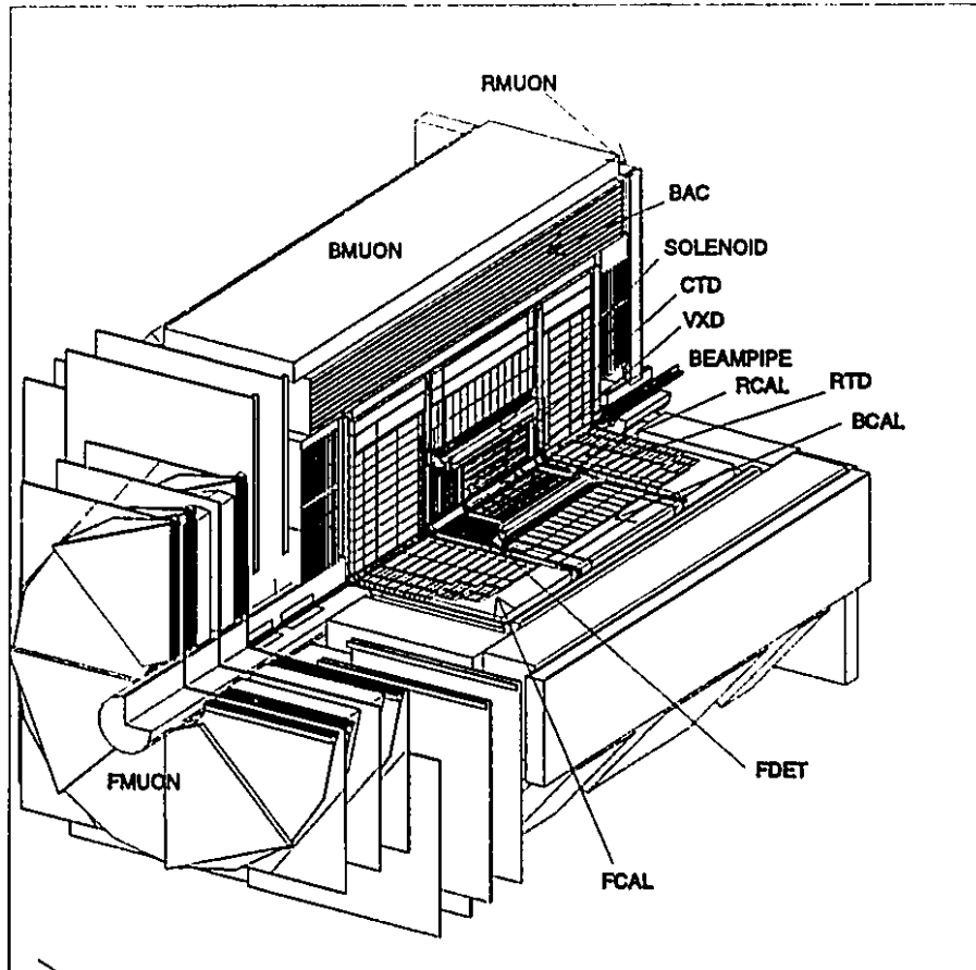
Figure 2.2: The components of the ZEUS detector, showing in particular the vertex detector (VXD) next to the beam pipe, the central tracking detector (CTD) which surrounds the VXD and is encased in a solenoidal magnet (SOLENOID) which provides a 1.43 T magnetic field. Surrounding the CTD are the forward, barrel and rear calorimeters (FCAL, BCAL and RCAL respectively).
