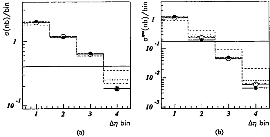
Figure D.4: Unfolding of the \Delta\eta distributions of a pure resolved Monte Carlo sample using the mixed Monte Carlo sample inputs. The inclusive distribution is shown in (a) and the distribution of gap events is shown in (b). The solid line shows the starting distribution. The dashed, dotted and dashed-dotted lines show the first, second and third iterations respectively. The solid line shows the result of the final iteration. The open circles show the hadron-level distributions.
