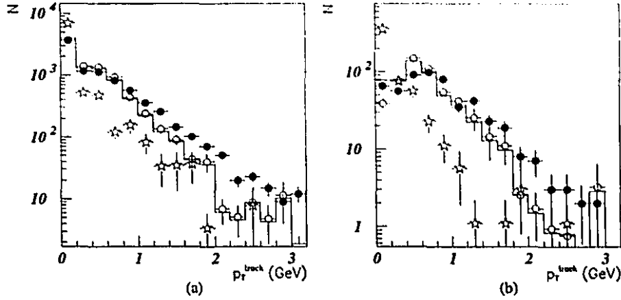
Figure 4.15: The p_T^{track} distribution of the maximum p_T^{track} track between the jets. The ZEUS data are shown by black dots. The prediction by the PYTHIA non-singlet sample is shown by the open circles and the prediction by the PYTHIA singlet sample is shown by the stars. The prediction by the PYTHIA mixed sample is shown by the solid line. In (a) the distribution is shown for all events and in (b) the distribution is shown just for the subsample with \Delta\eta > 3.5 .
