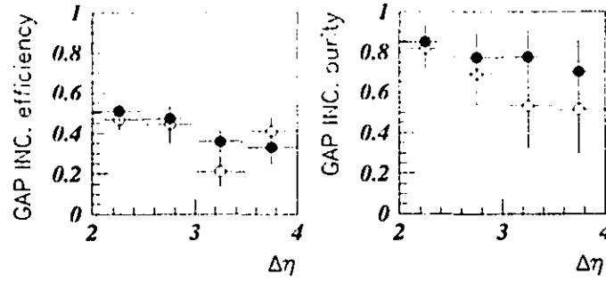
Figure 5.12: Gap efficiency and purity for a “tight” gap definition. The incremental bin-efficiency is shown on the left and the incremental bin-purity is shown in the right. The non-singlet PYTHIA sample is shown by the open circles and the mixed PYTHIA sample is shown by the black dots.
