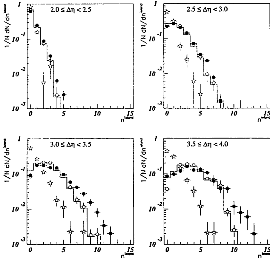
Figure 5.1: The island multiplicity distributions in four bins of \Delta\eta . The data are shown as black dots. The prediction by the PYTHIA events with no colour singlet exchange (the non-singlet sample) is shown by open circles and the prediction by the PYTHIA sample which contains only electroweak quark quark scattering (the singlet sample) is shown by stars. The solid line shows the prediction of the PYTHIA events with 10% of colour singlet exchange processes (the mixed sample).
