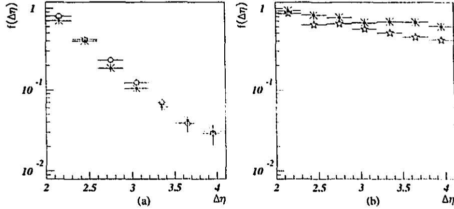
Figure 5.7: Gap-fractions at the detector and hadron levels. In (a) the gap-fraction of the non-singlet sample is shown at the detector-level by open circles and at the hadron-level by asterixes. In (b) the gap-fraction of the singlet sample is shown. The detector-level gap-fraction is shown by stars and the hadron-level gap-fraction is shown by asterixes.
