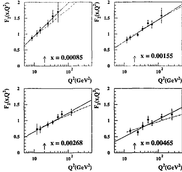
Figure 1.3: The F_2 structure function measurements of ZEUS together with linear fits (solid lines) and the results of a GLAP QCD fit (dashed-dotted lines). The inner error bars show the statistical error and the outer error bars show the systematic uncertainty added in quadrature.
