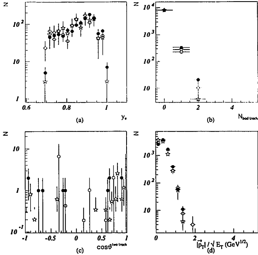
Figure 4.3: Cleaning quantities. The ZEUS data are shown by black dots. The prediction by the PYTHIA non-singlet sample is shown by the open circles and the prediction by the PYTHIA singlet sample is shown by the stars. The distribution of y_e for events with a scattered e^+ candidate in the calorimeter is shown in (a). In (b) one sees the number of rear pointing tracks. In (c) one sees the distribution of the cosine of the opening angle between the two tracks for events which have only two tracks and (d) shows the relative missing transverse momentum, |\vec{p}_T|/\sqrt{E_T} .
