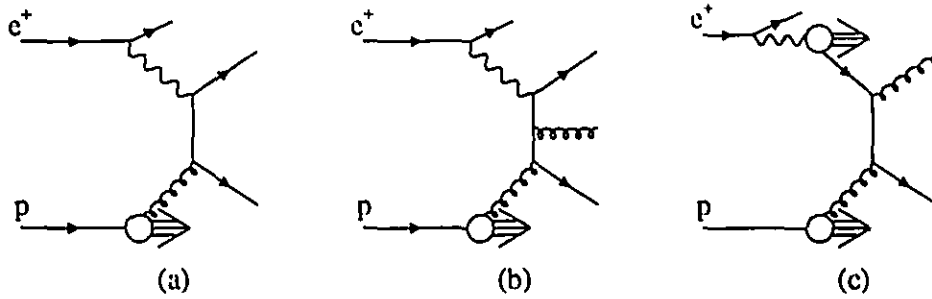
Figure 1.4: Diagrams for photoproduction at HERA. An example of a direct photoproduction process at leading order is shown in (a) while (b) shows a higher order direct photoproduction diagram. An example of a leading order resolved photoproduction process is shown in (c).
