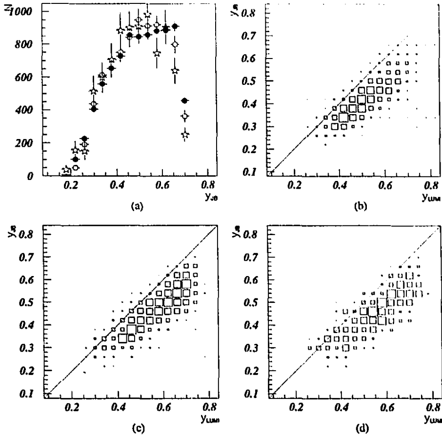
Figure 4.2: y_{JB} and y_{JB} versus y_{LUMI} . The ZEUS data are shown by black dots. The prediction by the PYTHIA non-singlet sample is shown by the open circles and the prediction by the PYTHIA singlet sample is shown by the stars. In (a) the distribution of y_{JB} is shown. One sees the correlation between y_{JB} and y_{LUMI} for the subsample of events in which the scattered e^+ is detected in the e^+ LUMI detector in (b), (c) and (d) for the data, the non-singlet sample and the singlet sample respectively.
