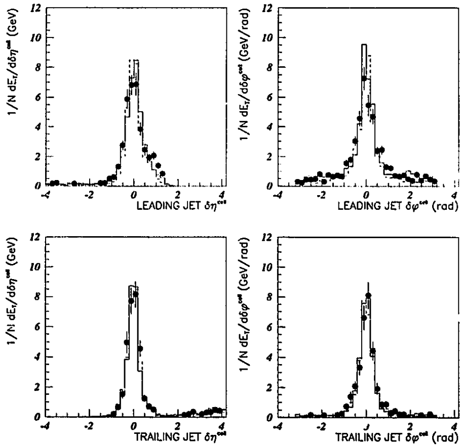
Figure 4.9: Jet profiles for the leading and trailing jets, for the gap candidate events with \Delta\eta > 3.5 . The data are shown as black dots. The predictions of the PYTHIA singlet and non-singlet samples are shown by the solid and dashed lines respectively.
