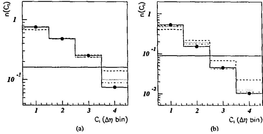
Figure D.3: Unfolding of the mixed Monte Carlo \Delta\eta distributions using the mixed Monte Carlo sample inputs. The unfolding of the inclusive distribution is shown in (a) and (b) shows the unfolding of the distribution of the gap events. The filled histogram shows the hadron-level \Delta\eta distributions. The solid line shows the starting distribution and the dashed, dotted and dashed-dotted lines show the first, second and third iterations of the unfolding procedure respectively. The final iteration of the unfolding procedure is represented by the black dots.
