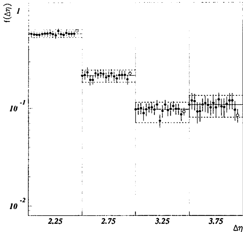
Figure 5.16: The gap-fraction computed in seventeen different ways (see text) is shown by the black dots and the white dots show the gap-fraction before the detector corrections for comparison.
