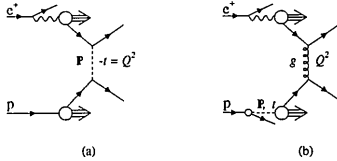
Figure 1.6: In (a) a hard diffractive scattering process is shown which proceeds via exchange of a colour singlet object, labelled P , of virtuality t = -Q^2 . The complementary diffractive hard process is shown in (b). The colour singlet object, P , has a small virtuality t , while the hard energy scale Q^2 comes from the virtuality of the exchanged gluon, g .
