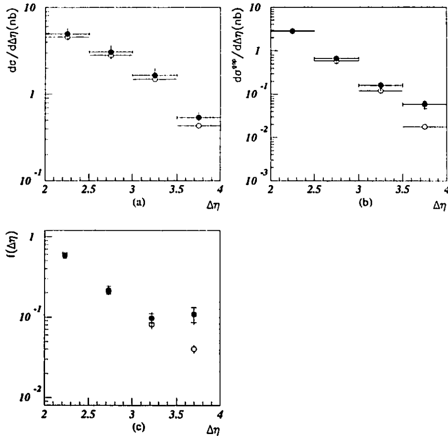
Figure 6.1: The data (corrected for detector effects) are shown as black dots where the inner error bar shows the statistical error and the outer error bar shows the systematic uncertainty added in quadrature. The predictions of the PYTHIA non-singlet sample for the hadron-level distributions are shown as open circles. The inclusive cross section is shown in (a). The gap cross section is shown in (b) and the gap-fraction is shown in (c).
