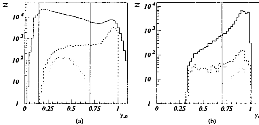
Figure 3.4: Distribution of the y estimators. The solid line shows a loose sample of dijet events. The dashed line shows the sample of dijet events which will be used in this analysis and the dotted line shows a clean sample of photoproduction events where the scattered e^+ is measured in the e^+ LUMI detector. y_{JB} , which is estimated using the hadronic energy deposits in the calorimeter, is shown in (a) and y_e , which is estimated using the energy deposits of a scattered e^+ candidate, is shown in (b).
