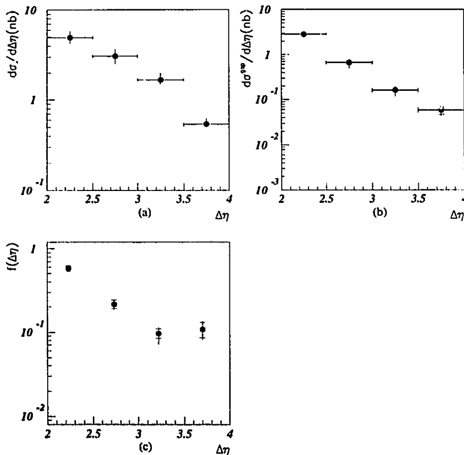
Figure 5.18: The cross section d\sigma/d\Delta\eta is shown in (a). The gap cross section d\sigma^{gap}/d\Delta\eta is shown in (b) and the gap-fraction, f(\Delta\eta) , is shown in (c). The corrected ZEUS data are shown as black dots. The inner error bars show the statistical errors (in some cases within the marker) and the outer error bars show the systematic uncertainties.
