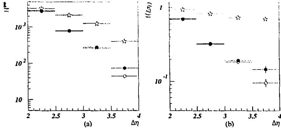
Figure 5.4: The \Delta\eta distribution for gap events where a gap is defined as no tracks with p_T^{\text{track}} > 250 MeV is shown in (a). The corresponding gap-fraction is shown in (b). The data are shown as black dots. The prediction by the PYTHIA non-singlet sample is shown by open circles and the prediction by the PYTHIA singlet sample is shown by stars.
