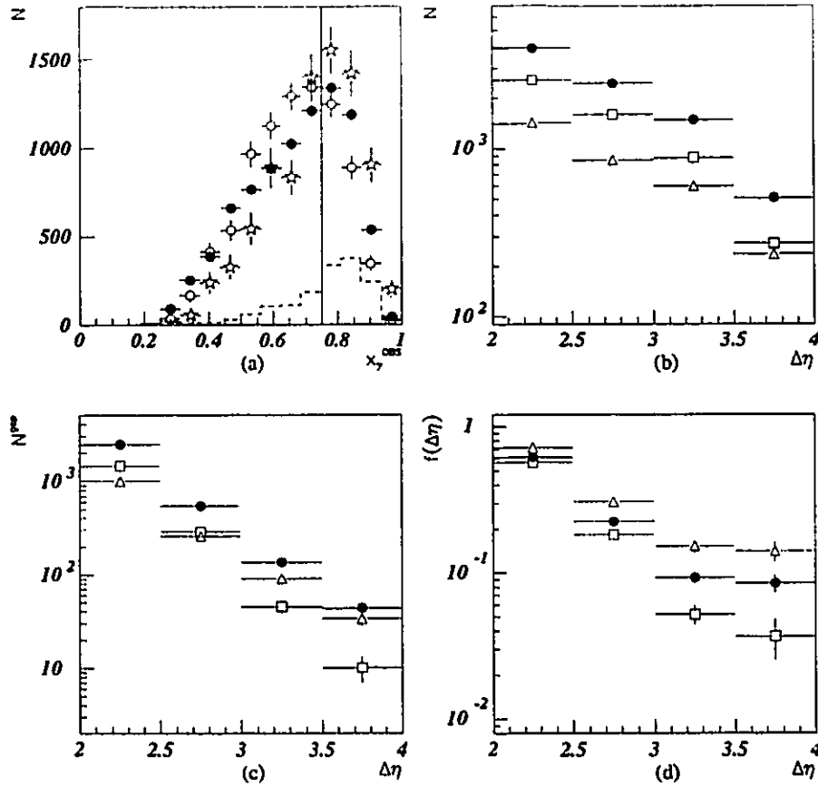
Figure 6.7: The dependence of the gap-fraction on x_{\gamma}^{\text{OBS}} . The distribution of x_{\gamma}^{\text{OBS}} is shown in (a). The data are shown as black dots. The PYTHIA sample containing no colour singlet exchange processes (the non-singlet sample) is shown as open circles. The subsample of the non-singlet sample which is due to LO direct processes is shown by the dashed line. The stars represent the PYTHIA sample which includes only colour singlet exchange processes (the singlet sample). The vertical line is drawn at x_{\gamma}^{\text{OBS}} = 0.75 . The inclusive \Delta\eta distribution, the \Delta\eta distribution for gap events, and the gap-fraction are shown in (b), (c) and (d) respectively. (These distributions are uncorrected for detector effects and the errors shown are statistical only.) In (b), (c) and (d) only the measured data are shown (black dots). The triangles show the x_{\gamma}^{\text{OBS}} \geq 0.75 subsample and the squares show the x_{\gamma}^{\text{OBS}} < 0.75 subsample.
