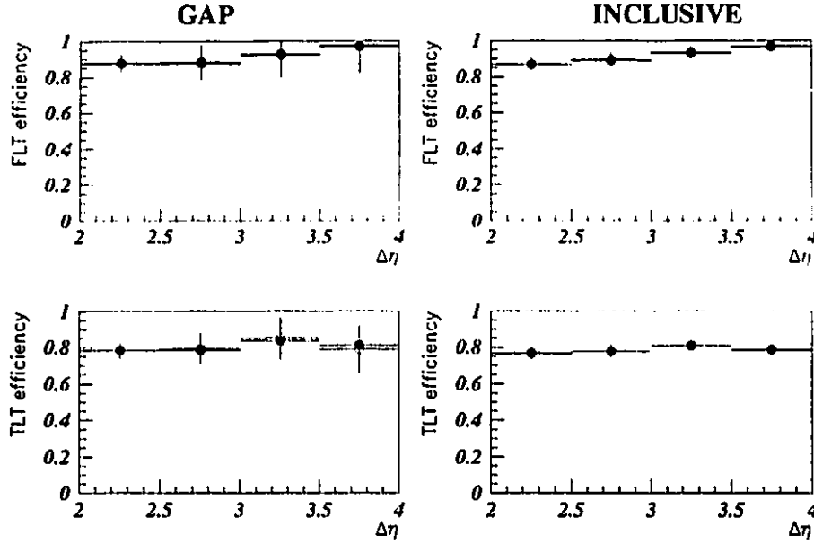
Figure 4.16: The FLT efficiency is shown in the first row and the cumulative trigger efficiency (up to the TLT) is shown in the second row. The efficiency for hadron-level gap events is shown in the left column and the inclusive efficiency is shown in the right column. The efficiencies according to the standard PYTHIA sample (the non-singlet sample) are shown as open circles and the efficiencies according to the PYTHIA sample with 10% colour singlet exchange processes (the mixed sample) are shown as black dots.
