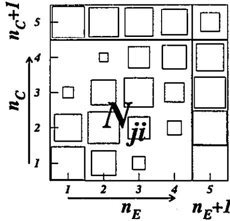
Figure D.1: Cause versus effect – Example of an unfolding problem.
