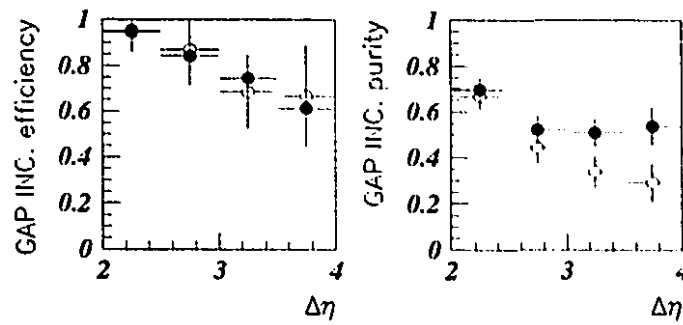
Figure 5.11: Gap efficiency and purity for a “loose” gap definition. The incremental bin-efficiency is shown on the left and the incremental bin-purity is shown in the right. The non-singlet PYTHIA sample is shown by the open circles and the mixed PYTHIA sample is shown by the black dots.
