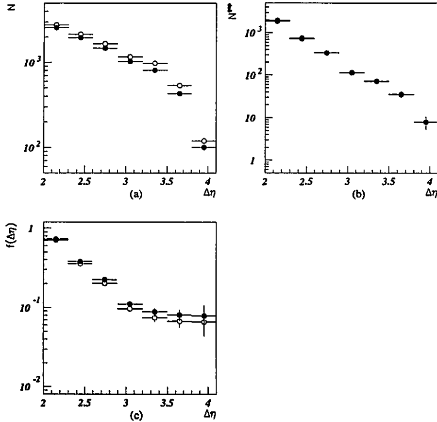
Figure C.2: The standard distributions calculated using the two jets of highest E_T^{jet} are shown as black dots. The inclusive \Delta\eta distribution, the \Delta\eta distribution for gap events and the gap-fraction are shown in (a), (b) and (c) respectively. The open circles show the corresponding distributions calculated using the jets at highest and lowest \eta^{jet} instead of the two highest E_T^{jet} jets.
