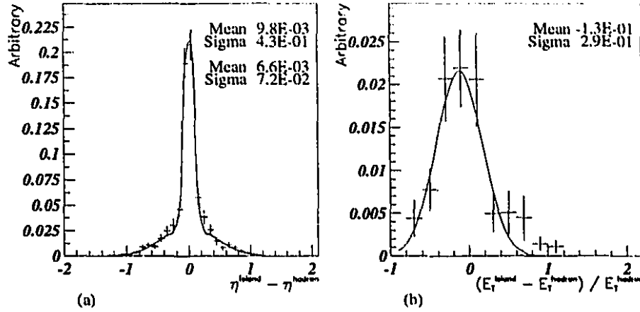
Figure 4.19: The resolution of \eta^{hadron} according to the PYTHIA mixed sample is shown in (a) and the resolution of E_T^{hadron} according to the PYTHIA mixed sample is shown in (b).
