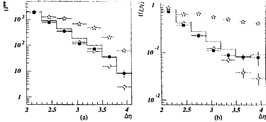
Figure 5.3: The uncorrected \Delta\eta distribution for gap candidates is shown in (a) and (b) shows the uncorrected gap-fraction. The data are shown as black dots. The prediction by the PYTHIA non-singlet sample is shown by open circles and the prediction by the PYTHIA singlet sample is shown by stars. The solid line shows the prediction of the PYTHIA mixed sample.
