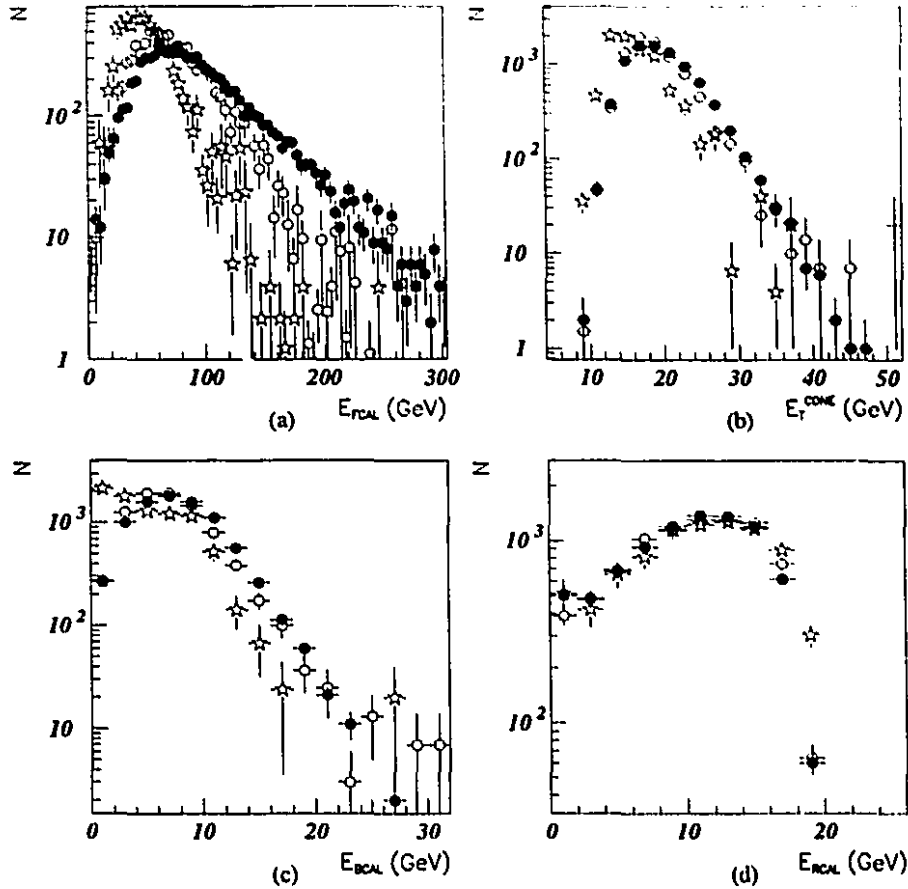
Figure 4.1: Global energy sums. The ZEUS data are shown by black dots. The prediction by the PYTHIA sample with no colour singlet exchange events (the non-singlet sample) is shown by the open circles and the prediction by the PYTHIA sample with only electroweak quark-quark scattering (the singlet sample) is shown by the stars. In (a) the distribution of the total energy deposited in the FCAL is shown. In (b) the distribution of the transverse energy outside a cone of 10^\circ is shown. In (c) one sees the distribution of the energy deposited in the BCAL and in (d) one sees the distribution of the energy deposited in the RCAL.
