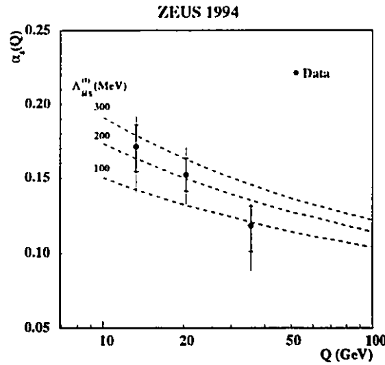
Figure 1.2: ZEUS measured values of \alpha_s(Q) for three different Q^2 regions. The statistical error corresponds to the inner bar and the thin bar shows the statistical and systematic uncertainties added in quadrature. The dashed curves show QCD predictions for the running of \alpha_s(Q) .
