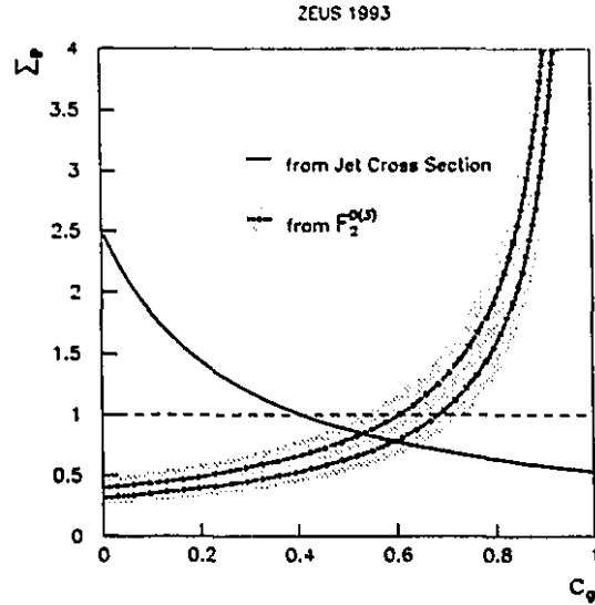
Figure 1.7: The plane of the variables \Sigma_p (sum of momenta of partons in the pomeron) and c_g (relative contribution of hard gluons in the pomeron). The solid line is obtained from a \chi^2 fit to the inclusive jet cross section of Monte Carlo predictions for the pomeron structure. The dashed dotted lines show the constraint imposed by the measurement of the diffractive structure function in DIS.
