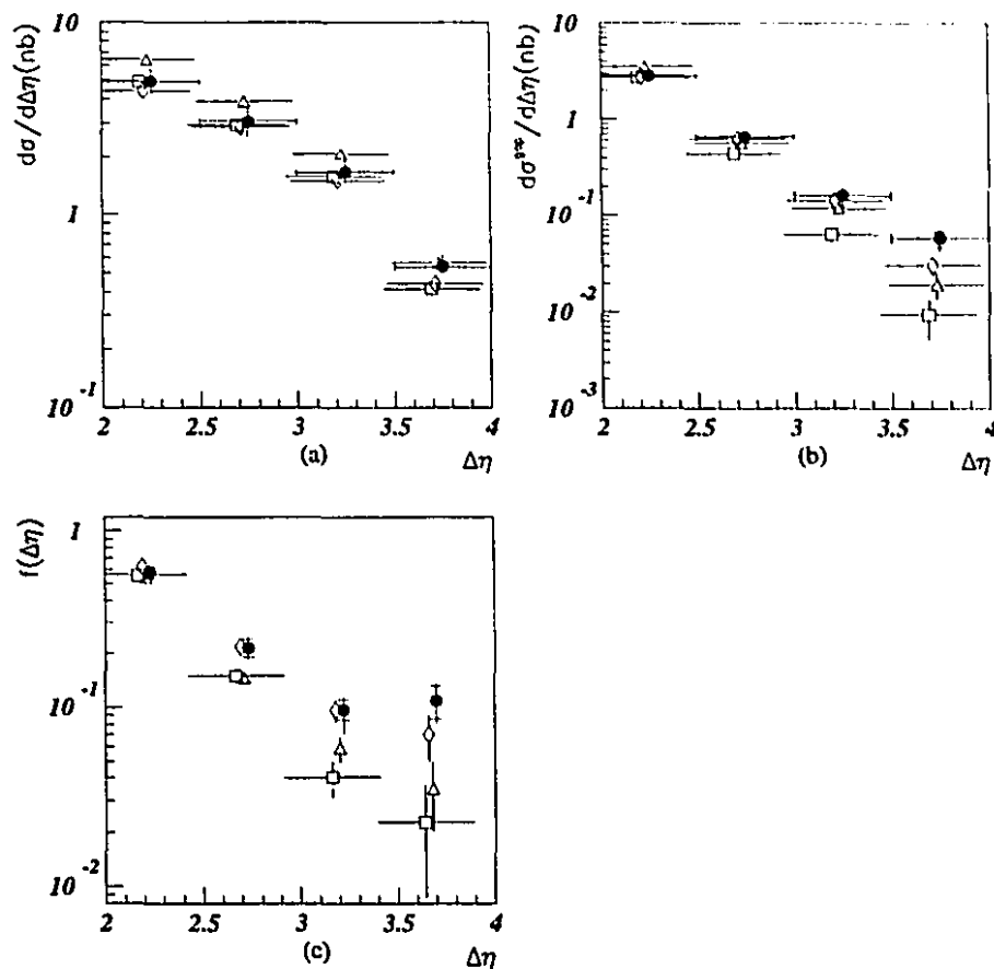
Figure 6.2: The data (corrected for detector effects) are shown as black dots where the inner error bar shows the statistical error and the outer error bar shows the systematic uncertainty added in quadrature. The PYTHIA predictions including multiple interactions are shown as triangles. The predictions using the Field-Feynman fragmentation function are shown as squares and the predictions from lowering \sigma_{pT} are shown as diamonds.
