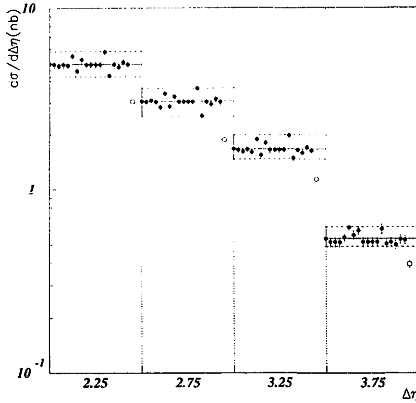
Figure 5.14: The inclusive cross section computed in seventeen different ways (see text) is shown by the black dots and the white dots show the distribution before the detector corrections for comparison.
