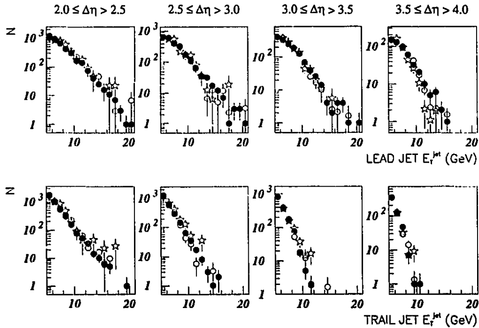
Figure 4.11: The E_T^{jet} distribution of the leading and trailing jets in four bins of \Delta\eta . The ZEUS data are shown by black dots. The prediction by the PYTHIA non-singlet sample is shown by the open circles and the prediction by the PYTHIA singlet sample is shown by the stars.
