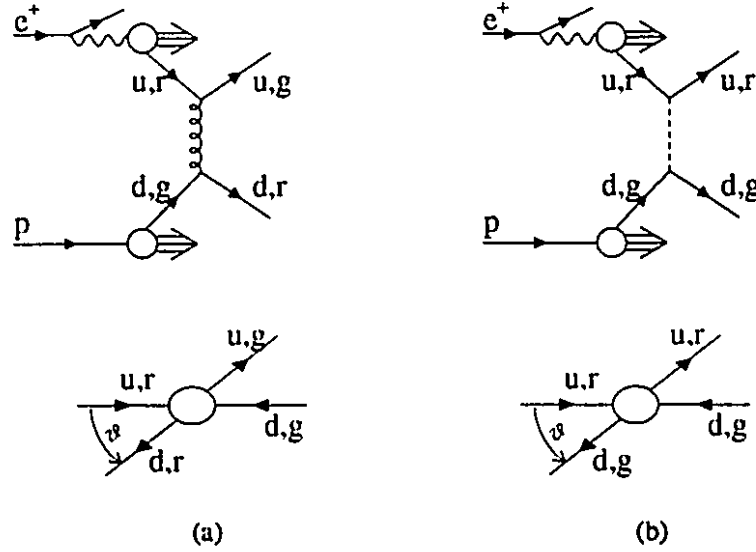
Figure 1.8: Two examples of the colour flow in hard photoproduction events at HERA. In the top view the full schematic diagram of the process is shown and in the bottom view just the hard subprocess is shown, in its centre-of-mass frame. An example of a colour non-singlet exchange event is shown in (a) and an example of a colour singlet exchange event is shown in (b).
