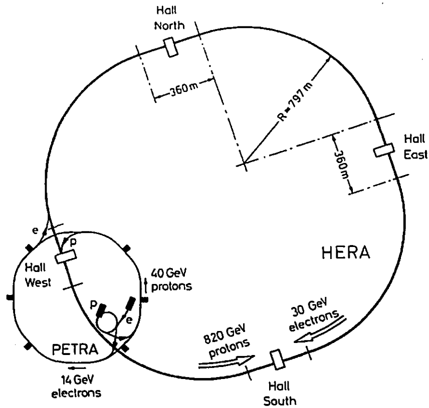
Figure 2.1: The layout of the HERA accelerator complex, showing the p and e^+ linacs, the sequence of preaccelerators, and the HERA ring, with the four experimental halls.
