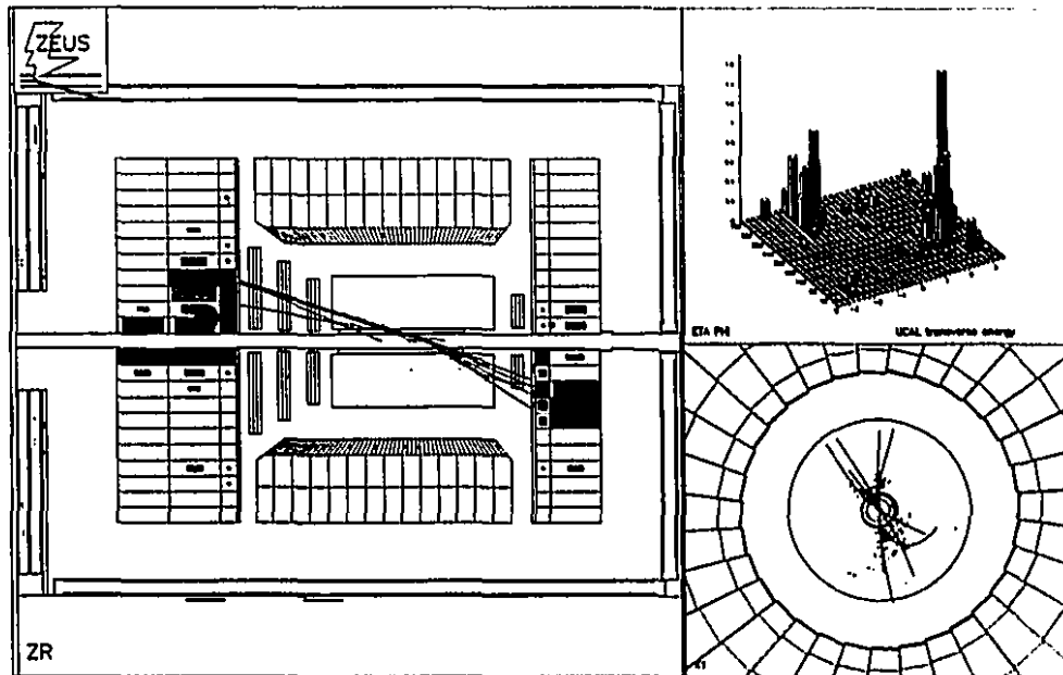
Figure 3.1: A dijet photoproduction event as seen by the ZEUS detector. The left side shows the rz view of the reconstructed tracks and the energy deposits in the calorimeter. The upper right view shows the energy deposits in the calorimeter in the \eta, \varphi plane and the lower right picture shows the xy view of the reconstructed tracks.
