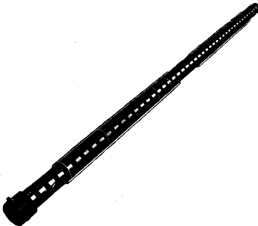
Fig. 3.5 The first T-Stick prototype before being covered, showing the strips of copper tape used as key electrodes for touch sensing.
