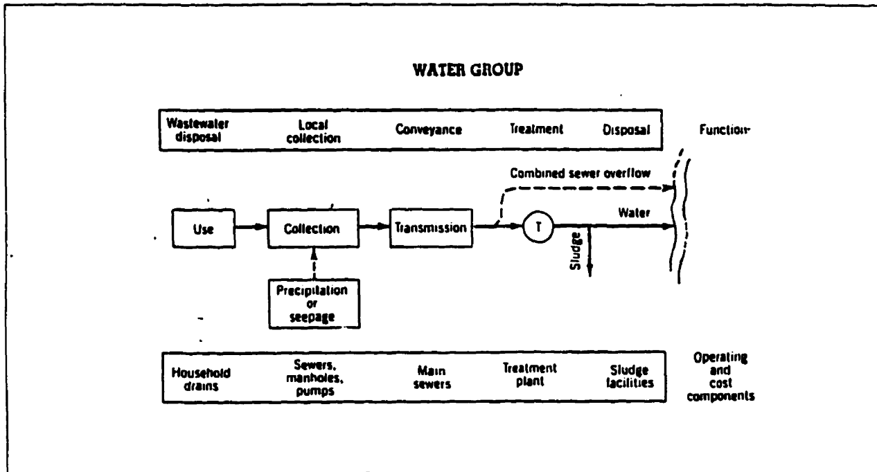
Figure 2.3 Configuration of an Urban Wastewater Management System (106)
