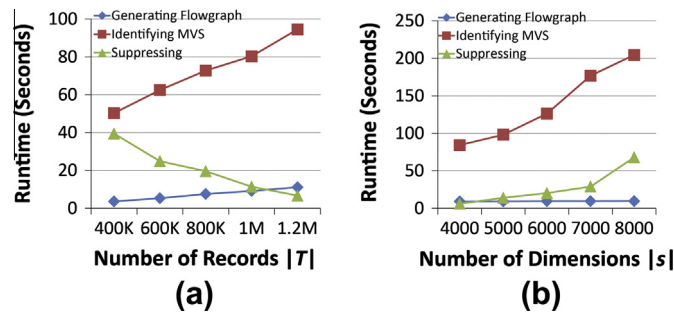
Fig. 7. Scalability.
