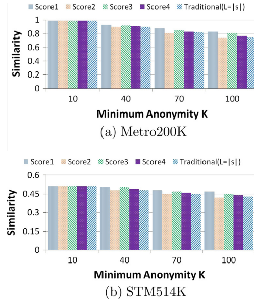
Fig. 4. Scenario I: Similarity vs. K ( L = 3 , w_\alpha = 0.5 , w_\beta = 0.3 , w_\gamma = 0.2 , w_\delta = 0 ).
