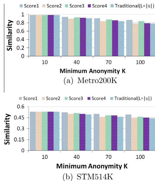
Fig. 6. Scenario III: Similarity vs. K ( L = 3 , w_\alpha = 0.25 , w_\beta = 0.25 , w_\gamma = 0.25 , w_\delta = 0.25 ).
