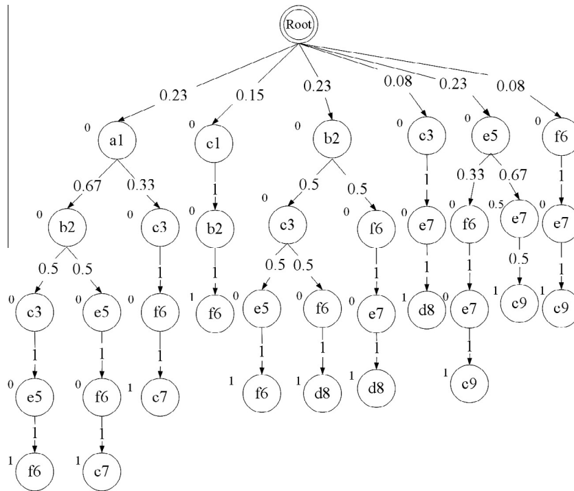
Fig. 2. LK-anonymized probabilistic flowgraph of Table 1.
