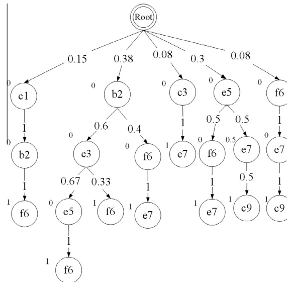
Fig. 3. K-anonymized probabilistic flowgraph of Table 1.
