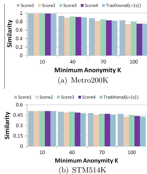
Fig. 5. Scenario II: Similarity vs. K ( L = 3 , w_\alpha = 0.3 , w_\beta = 0.5 , w_\gamma = 0.2 , w_\delta = 0 ).
