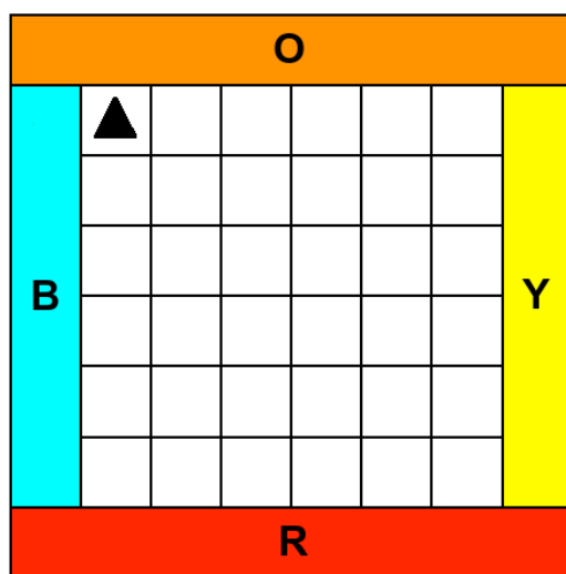
Figure 4.8: Grid World
