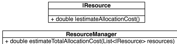
Figure 10.7: Allocation Cost Structural Design
