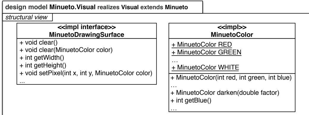
Figure 3.3: The Interface of the Feature Visual (sub-feature of Minueto )
