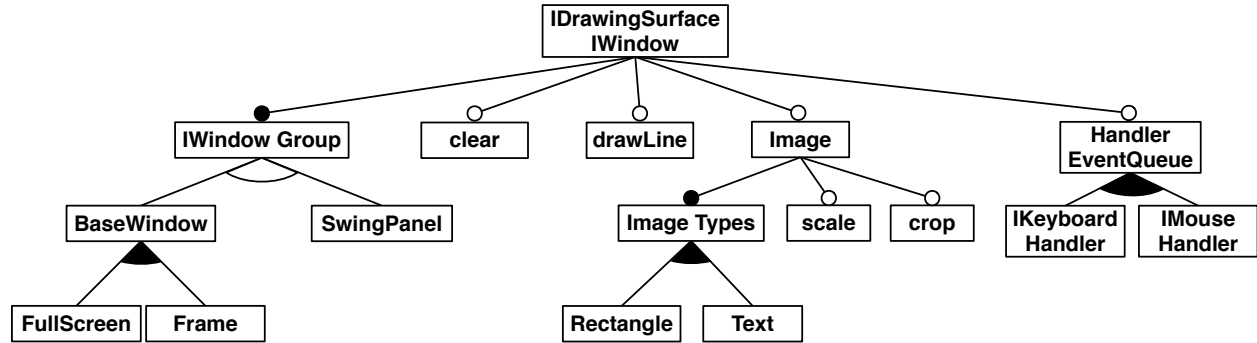
Figure 5.12: The Resulting Feature Model for the Running Example
