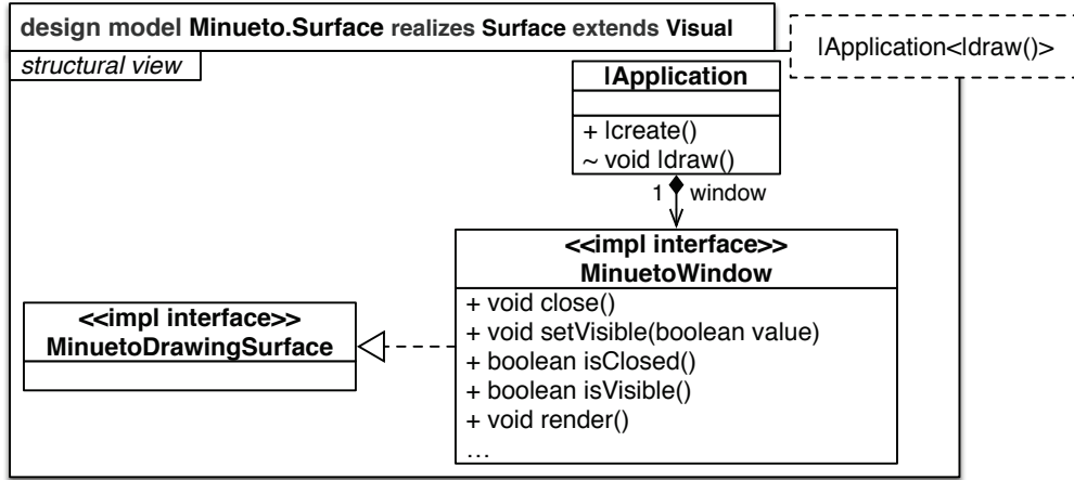
Figure 3.11: The Interface of the Feature Surface with Added Glue Code Structure
