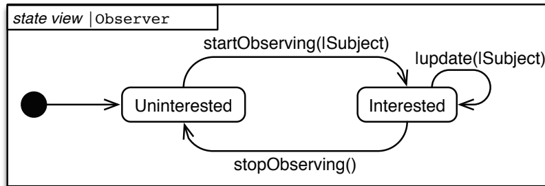
Figure 2.14: The State View for the Observer Class of the Base Feature of the Observer Concern.
