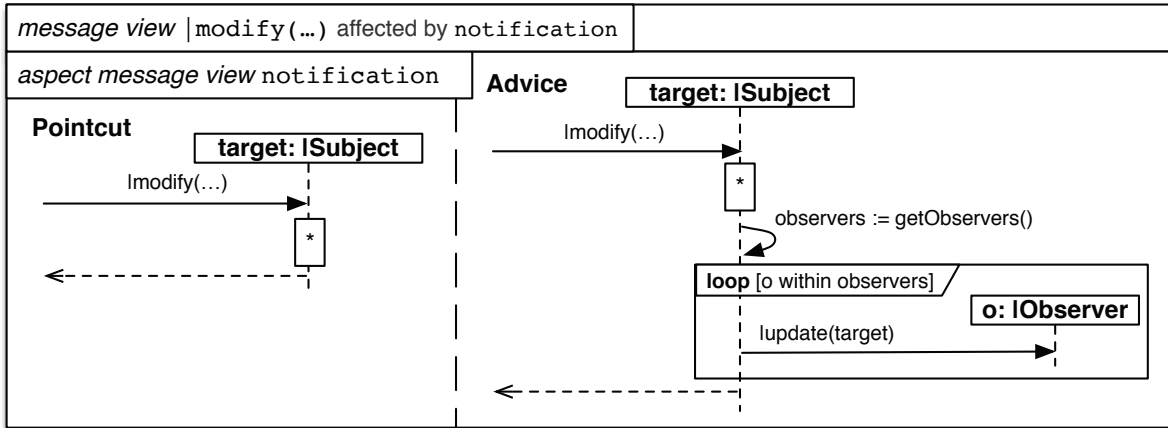
Figure 2.13: The Aspect Message View for Notifying Observers.
