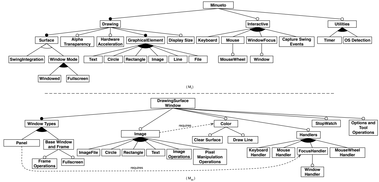
Figure 6.4: Minueto Feature Models of M_I (top) and M_{ac} (bottom)
