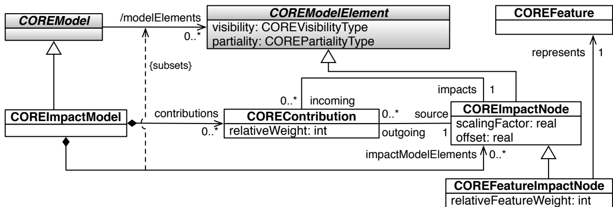
Figure 2.6: The Impact Model part of the CORE Metamodel.
