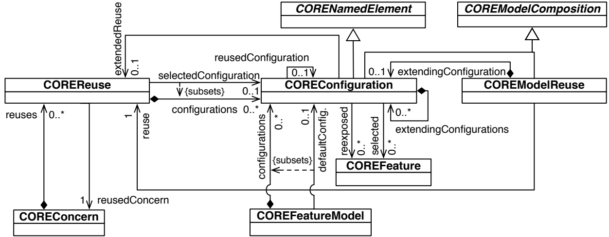
Figure 2.8: The Reuse part of the CORE Metamodel.
