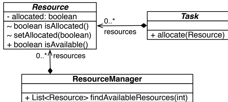
Figure 8.1: Resource Management Base Design
