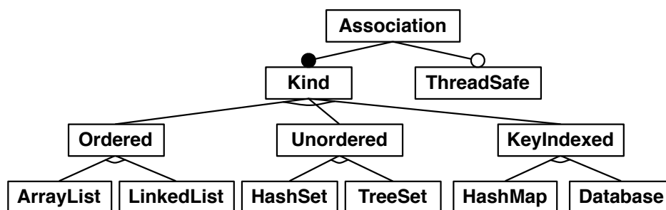
Figure 8.3: Association Feature Model
