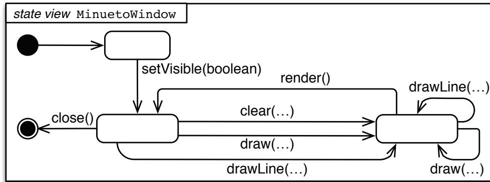
Figure 3.8: The Protocol Model of the Feature Surface for the MinuetoWindow Interface
