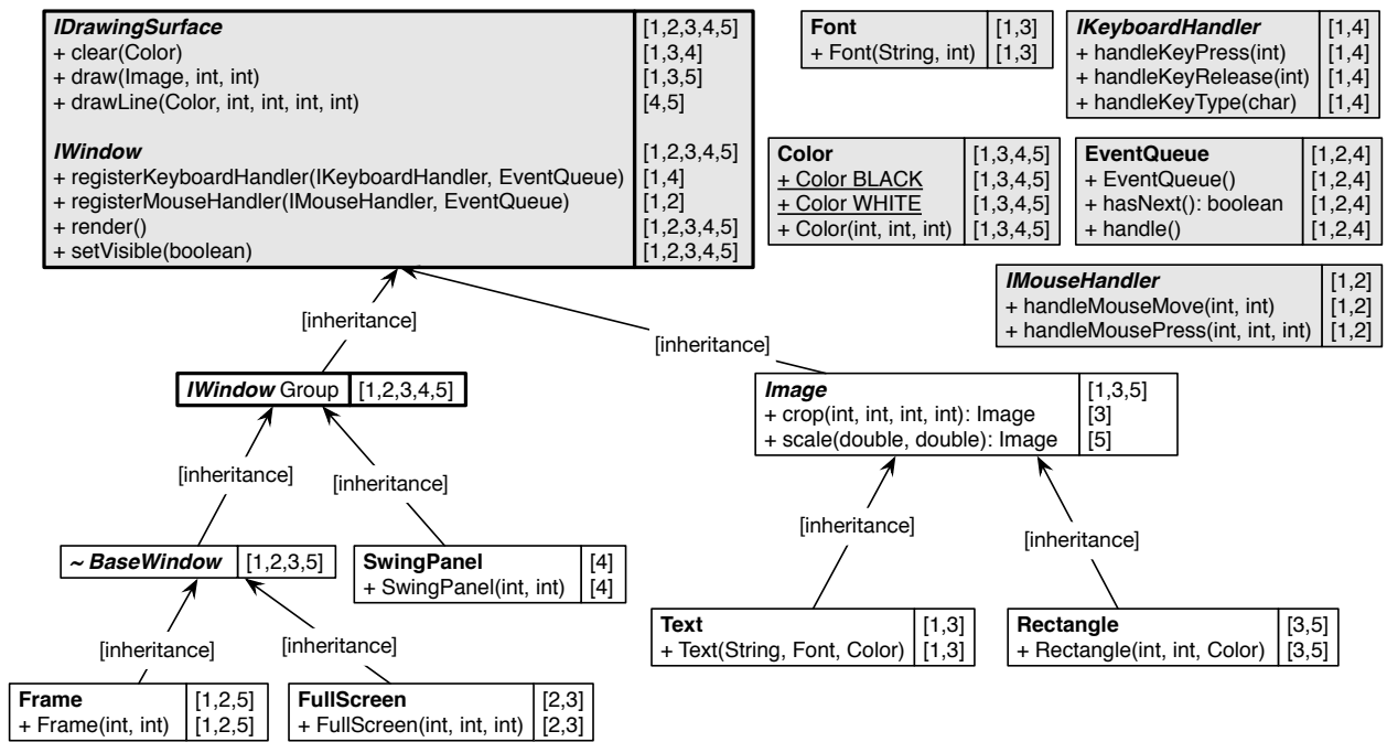
Figure 5.5: Intermediate result after simplifying hierarchies (updated nodes highlighted with thick stroke)
