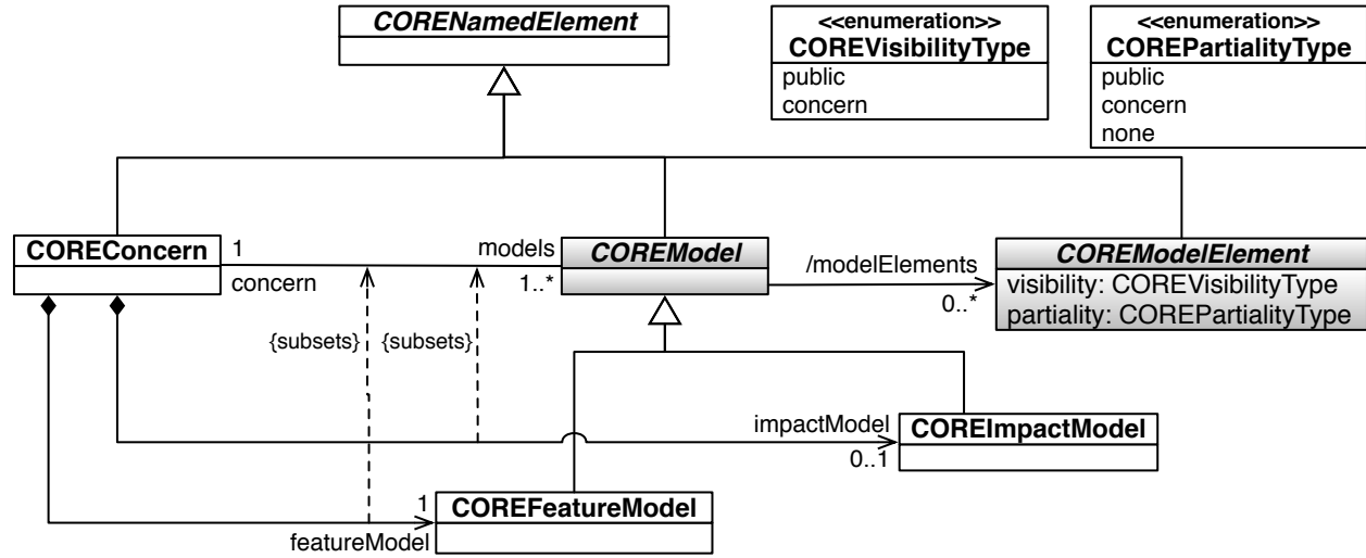
Figure 2.4: General Overview of a Concern in the CORE Metamodel.
