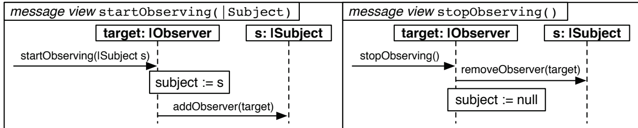
Figure 2.12: The Message Views for the Observer Feature of the Observer Concern.
