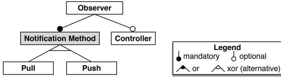
Figure 2.2: The Feature Model of the Observer Concern.
