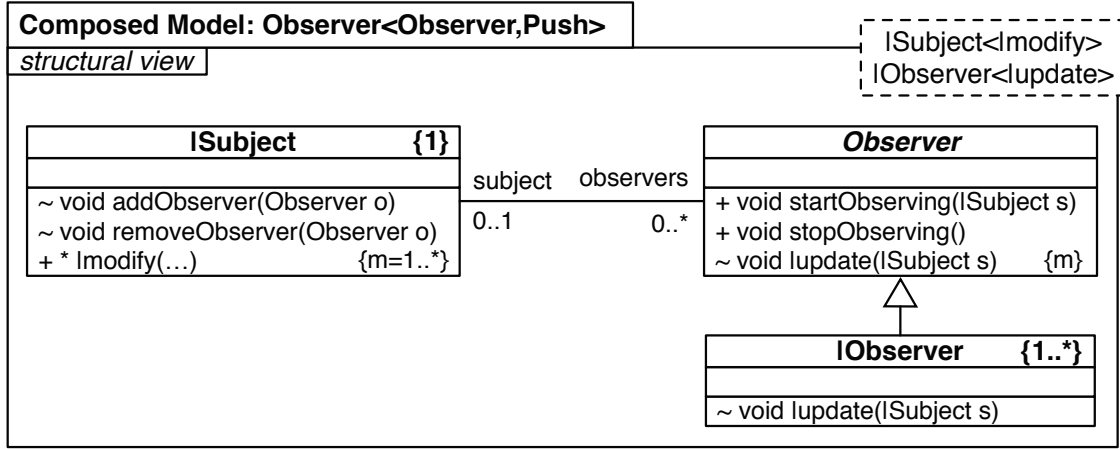
Figure 2.16: The Composed Model of the Observer Concern including Mapping Cardinalities.
