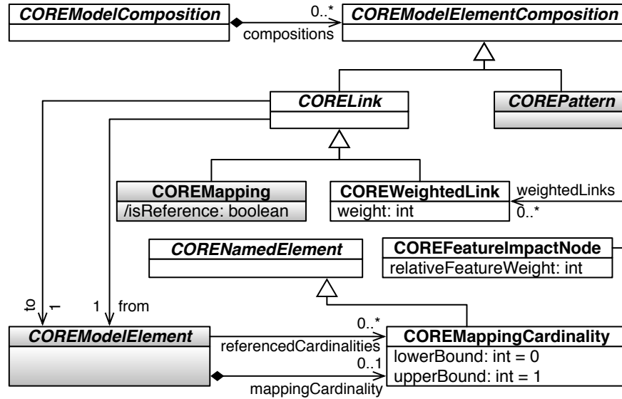
Figure 2.9: The Model Element Compositions part of the CORE Metamodel.
