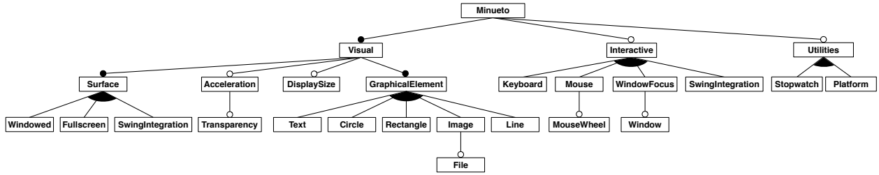
Figure 4.8: The initial feature model I_1 elaborated by the investigator
