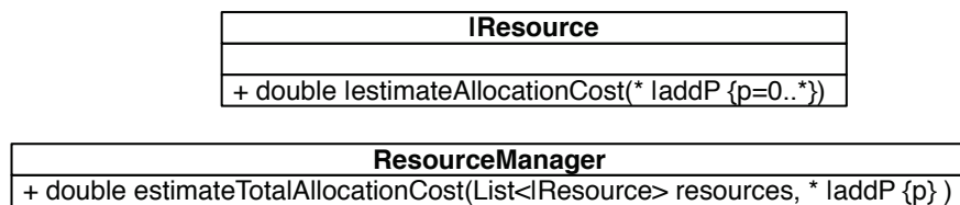
Figure 10.9: Updated Allocation Cost Structural Design
