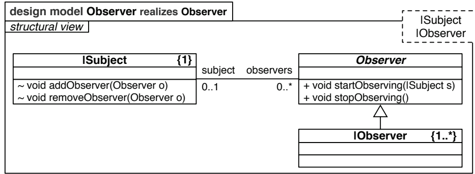
Figure 2.15: The Structural View for the Observer Feature of the Observer Concern with Mapping Cardinalities.
