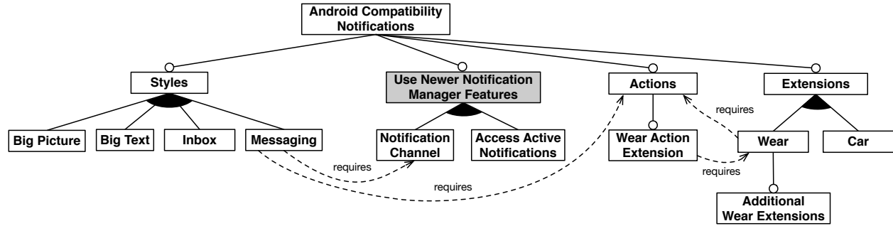
Figure 6.5: Android Notifications Feature Model determined by Automated Concernification
