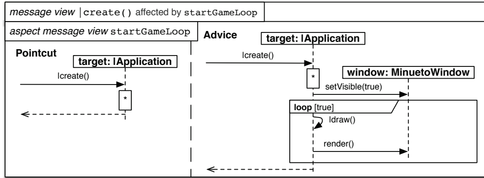
Figure 3.12: The Partial Glue Code Behaviour of the Feature Surface
