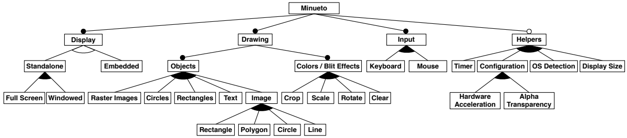
Figure 4.6: The updated feature model of D2 elaborated during the interview ( D2_2 )
