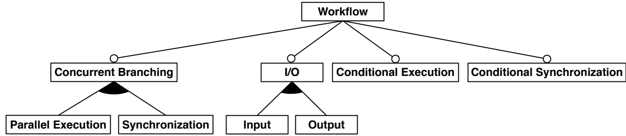
Figure 6.1: Workflow Feature Model
