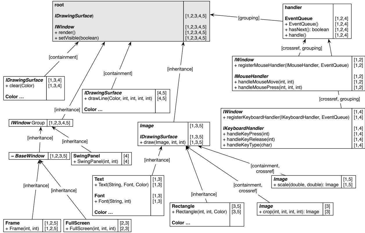
Figure 5.11: Final result after the edge simplification (root shown in grey)
