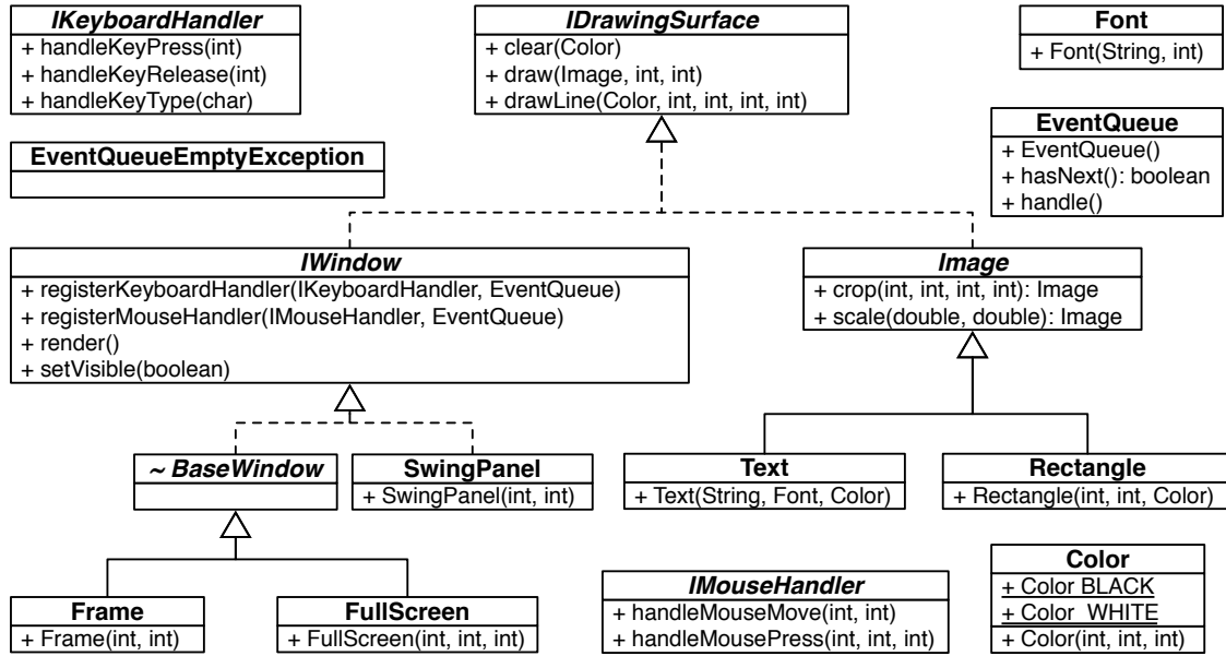
Figure 5.2: Class Diagram of Running Example
