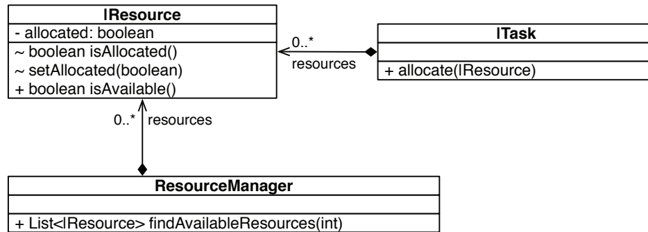
Figure 10.2: Resource Management Base Design
