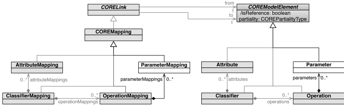
Figure 9.1: Class Diagram Metamodel Excerpt for Mappings and Classes
