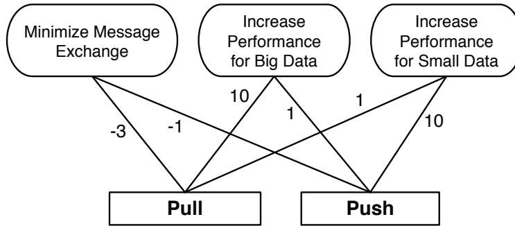
Figure 2.3: The Impact Model of the Observer Concern.
