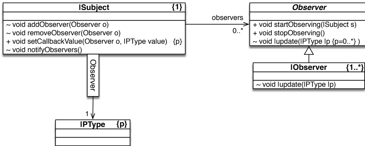
Figure 9.3: Supporting Custom Callback Values in the Observer
