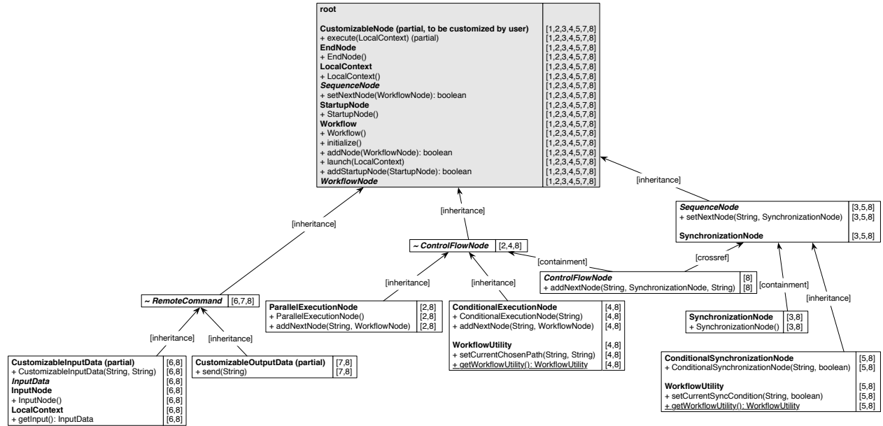
Figure 6.3: Resulting Graph of Workflow after Automated Concernification
