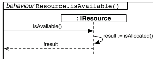
Figure 10.3: Behaviour for Checking the Availability of a Resource
