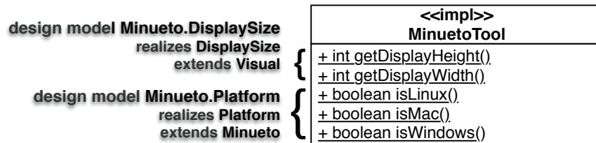
Figure 3.6: The Interface of the Class MinuetoTool and the Relation of its Methods to Features
