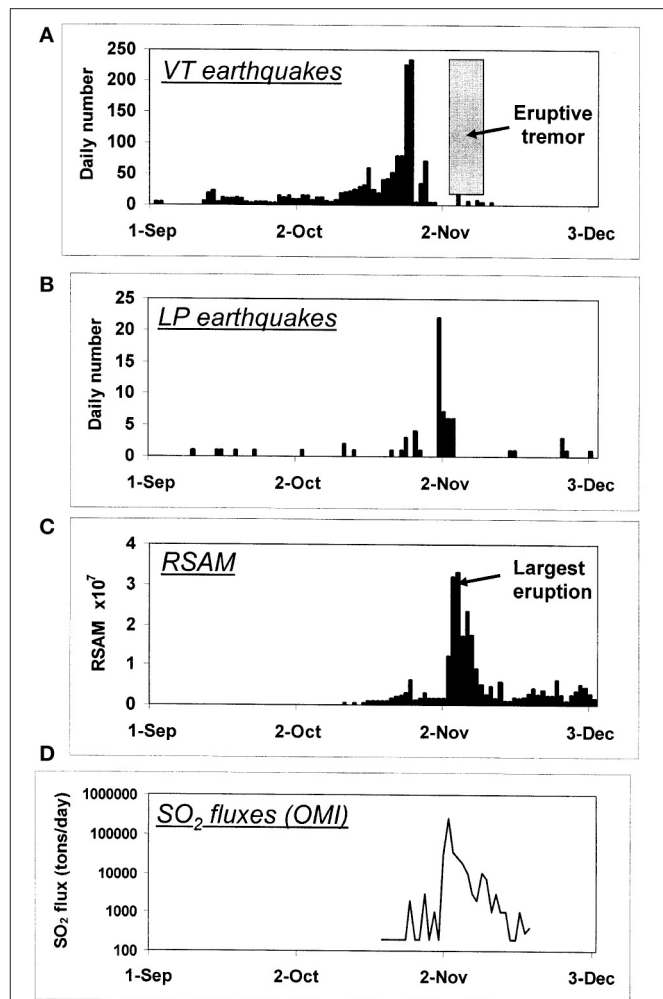
FIGURE 2 | Earthquakes and SO 2 fluxes at Merapi, September–November 2010. Note the appearance of volcanotectonic (VT) earthquakes in September 2010, their escalation in early-mid October, and their rapid decline by the end of October. Long-period (LP) earthquakes are clustered in latest October and earliest November. The paroxysmal eruptive phase during 3–5 November is associated with maximum RSAM, maximum SO 2 output, and the occurrence of eruptive tremor. Surono et al. (2012), Copyright 2012, with permission from Elsevier.
