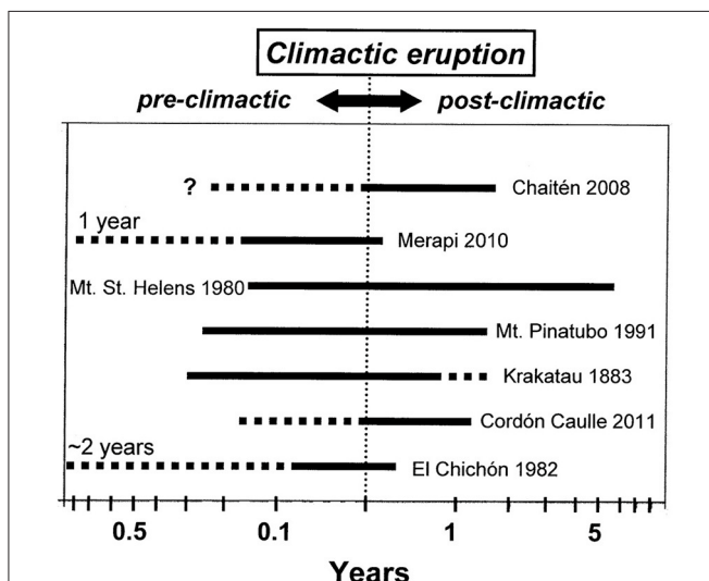
FIGURE 1 | Timescales of activity at fast volcanic systems, including precursory activity, climactic activity, and waning activity. Dashed lines indicate uncertainty in durations. For Chaitén, Pinatubo, and Krakatau, the degree of uncertainty is larger because these volcanoes were not monitored prior to the climactic eruptions.
