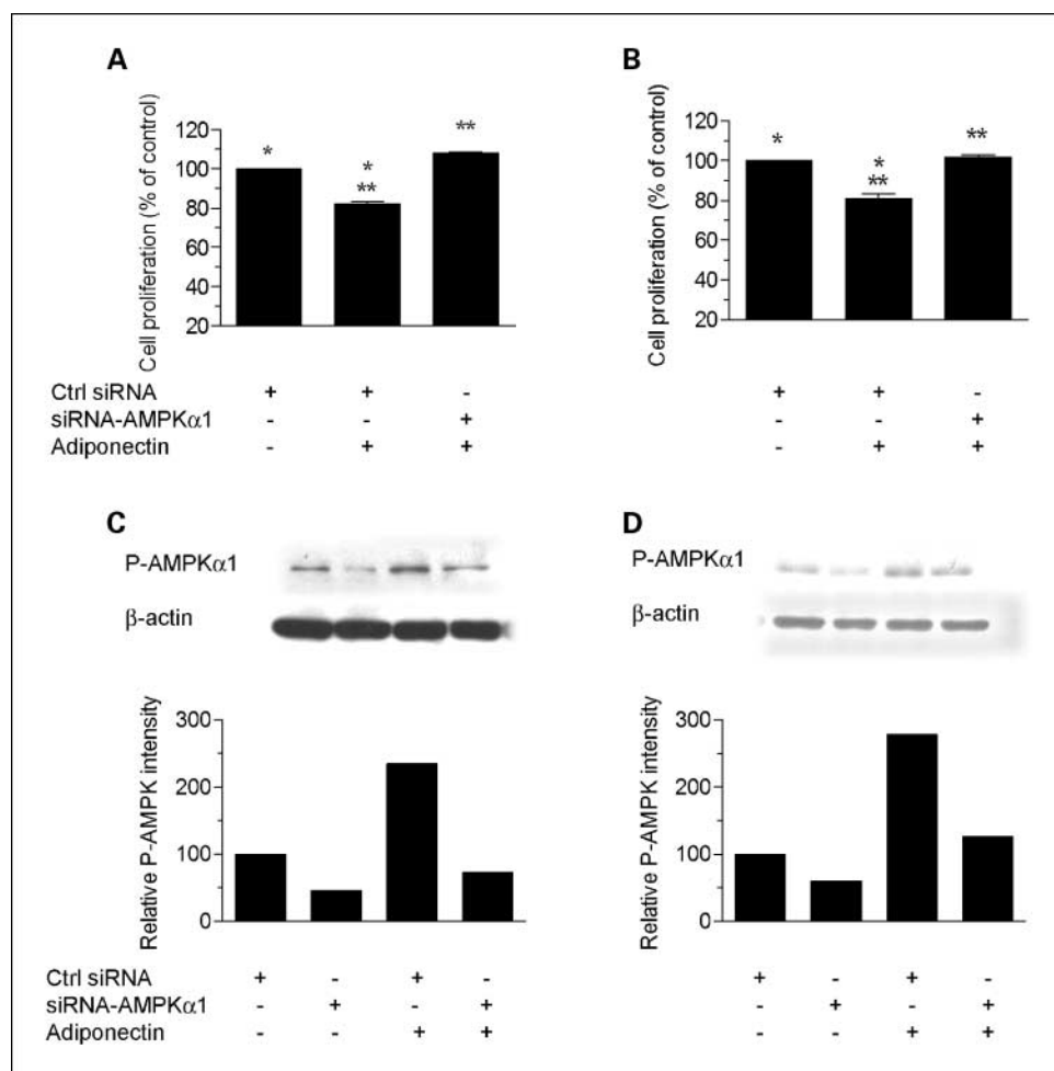
Fig. 3. AMPKα1 siRNA reduces phospho-AMPK levels and rescues cells from the inhibitory effect of adiponectin. Cell proliferation: HT-29 (A) and PC-3 (B) cells were transfected with 50 nmol/L AMPKα1-siRNA or with control siRNA (using MicroPore MP-100). Twenty-four hours after transfection, cells were treated with adiponectin (500 ng/mL) for 72 h. Cell proliferation in each well was measured by Alamar Blue dye reduction. Columns, mean of two independent experiments carried out in triplicate ( n = 6); bars, SE. *, significant difference between control and control plus adiponectin for both HT-29 ( P = 0.0017) and PC-3 ( P = 0.0077) cells. **, significant difference between siRNA-AMPK and siRNA-AMPK plus adiponectin for both HT-29 ( P = 0.0006) and PC-3 ( P = 0.0058) cells. Results are shown as the percentage of cell proliferation relative to control. Immunoblotting: HT-29 (C) and PC-3 (D) cells were transfected with 50 nmol/L AMPKα1-siRNA or with control siRNA; 24 h after transfection, adiponectin (500 ng/mL) was added and cells were incubated for 72 h. Cells were lysed and prepared for immunoblot analysis with antibodies against phospho-AMPK (Thr 172 ). β-Actin is shown as a loading control.
