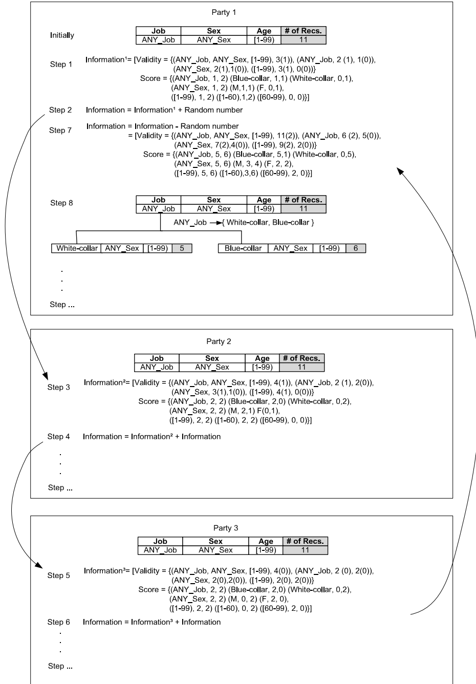
Fig. 4. Distributed anonymization.
