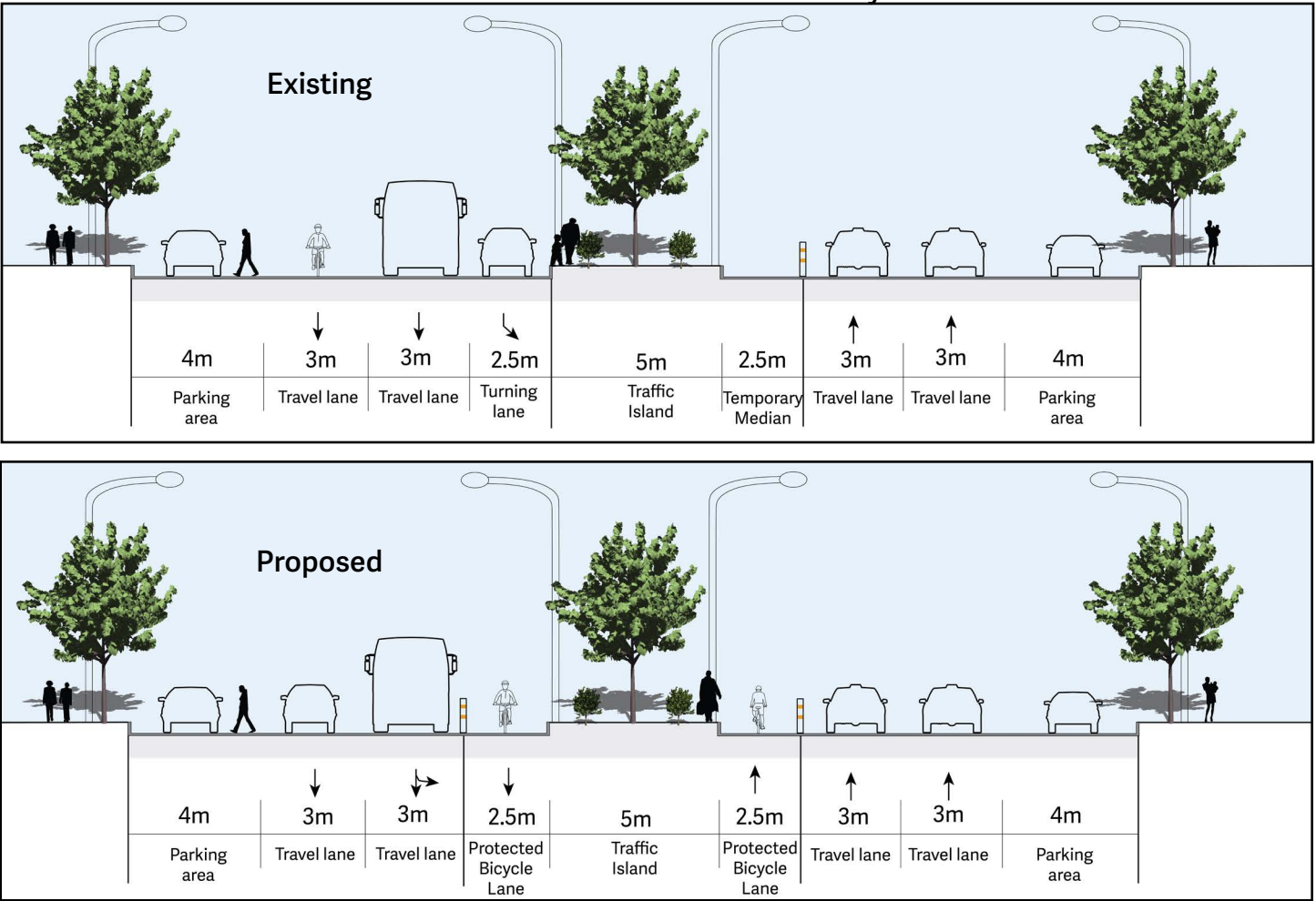
Adam Clayton Powell Jr. Blvd Cross-section
