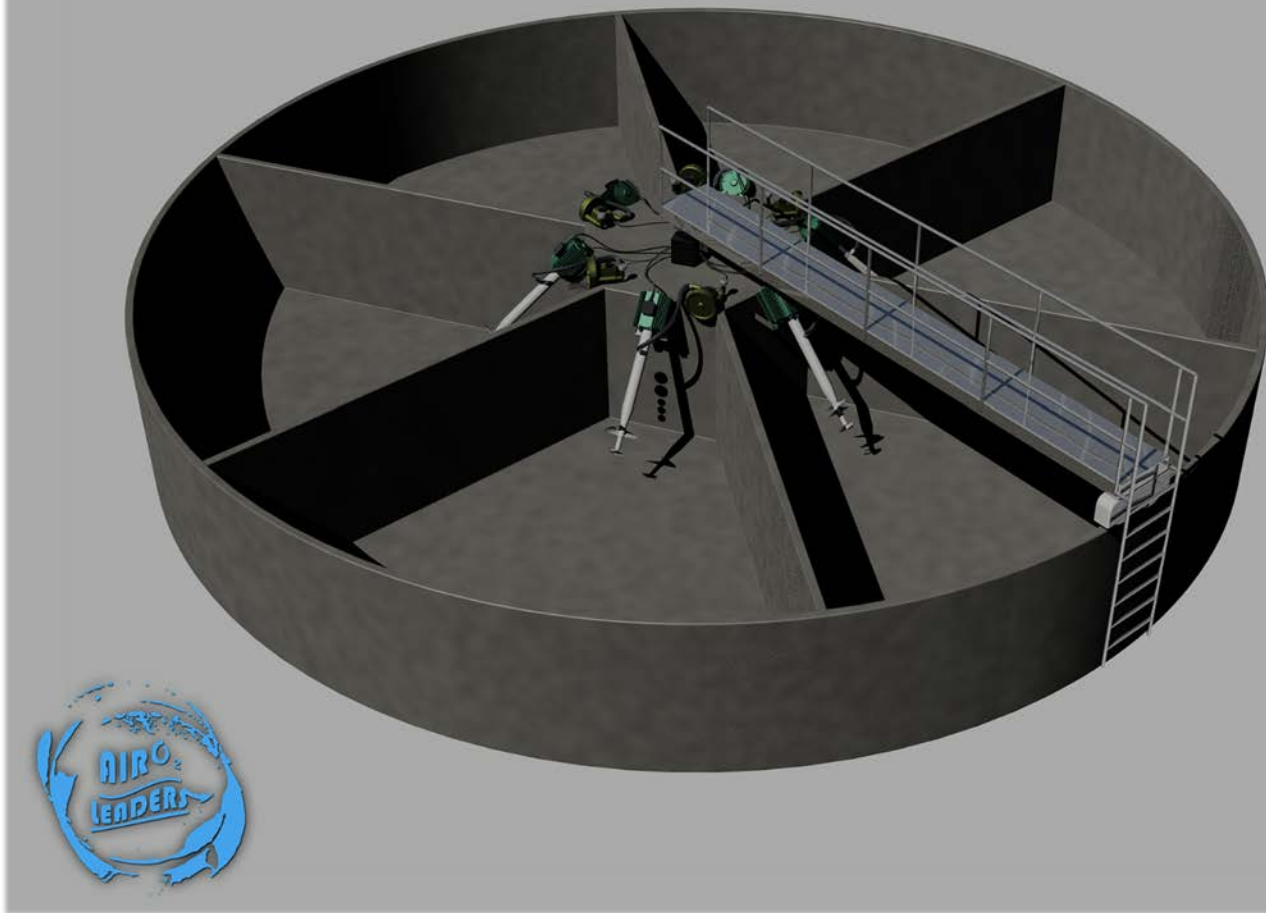
Figure 8. Mabarex Inc. provides the construction of the dual-cycle Hextuple compartment SBR (by Jun Dong)
