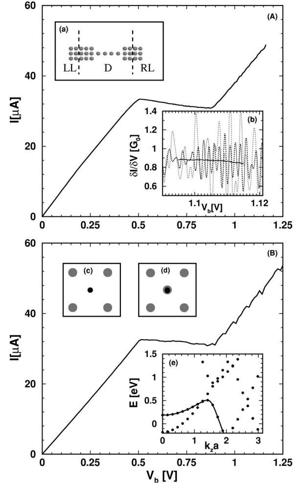
FIG. 3. I - V characteristics of Au contacts with hollow site registry (a) and top-site registry (b); with zero-bias conductance 0.94G_0 and 0.8G_0 for (a) and (b), respectively. The structure of the device is illustrated in (a), where LL, D, and RL correspond to left lead, effective device, and right lead, respectively. The hollow site is shown in (c) and top site in (d), where chain atoms are illustrated by dark circles. Inset (e) shows the band structure of the lead along the transport direction, the conducting band is shown by a solid line. Inset (b) shows differential conductance fluctuations of the Hollow site as a gray dotted line, dark dotted line, and dark continuous line for T=0 K, T=300 K and for T=300 K with 4 \times 10^{-3} V_{rms} modulation voltage taken into account, respectively.
