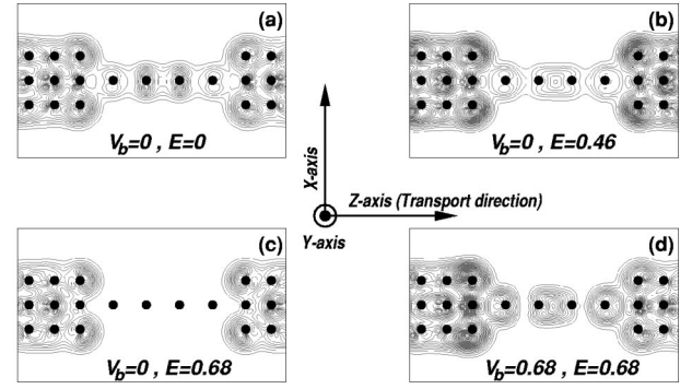
FIG. 4. Contour plots of surface charge density at particular bias voltage V_b (V) and energy E (eV) indicated on each figure. We use the same scale for all graphs to compare the conductance probability for each configuration. Dark circles correspond to atom positions along the constriction for guidance.
