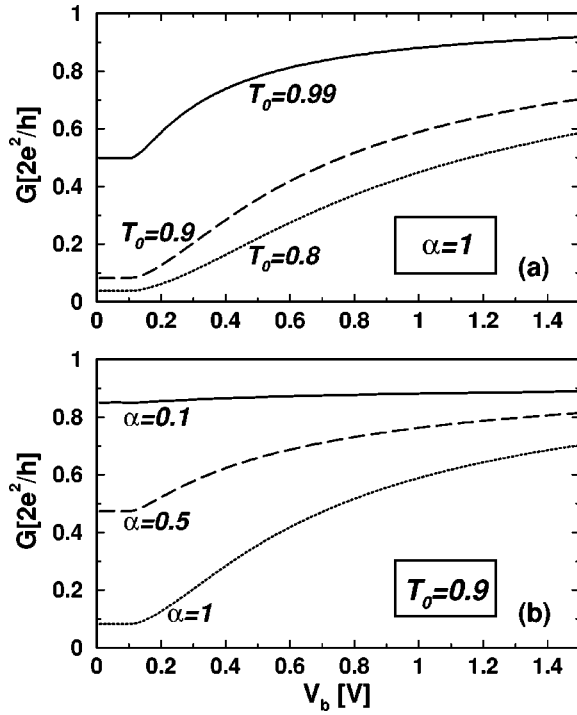
FIG. 9. Conductance calculated from renormalized transmission due to backscattering as a function of bias voltage (a) for T_0 = 0.99 , 0.9 , and 0.8 corresponding to solid, dashed, and dotted lines, respectively, with interaction parameter \alpha = 1.0 and (b) for T_0 = 0.9 and interaction parameter \alpha = 0.1 , 0.5 , and 1.0 corresponding to solid, dashed, and dotted lines, respectively.
