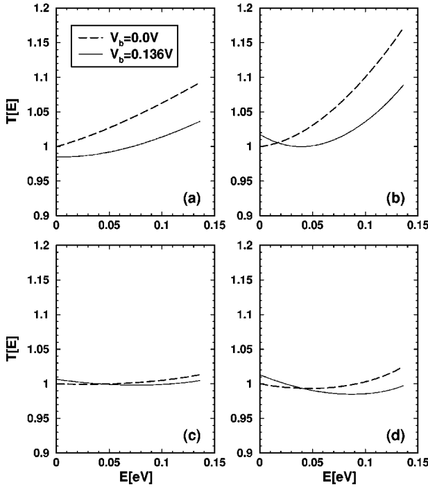
FIG. 7. Scaled transmission coefficient T(E) at V_b = 0 (dashed line) and V_b = 0.136 V (solid line) for ideal contact structure at the top site (a), one S impurity structure (b), disordered interface (c), and disordered interface with one S impurity (d). The scaling factor is T(E=0, V_b=0) .
