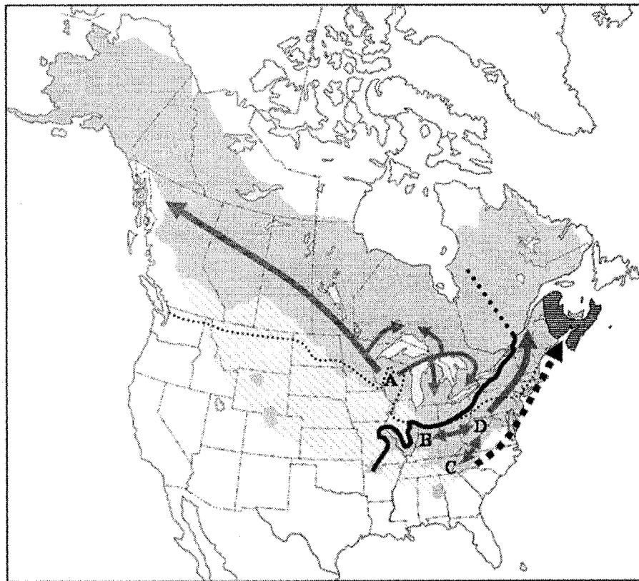
Figure 2.6. Summary of the post-glacial history of Rana sylvatica . The species' current range is shaded gray. Left slanting stripes indicating the potential historic extent of the range. The thin dotted line running east-west approximates the maximal southern extent of ice during the last glaciation. The solid black line indicates the boundary between eastern and western clades, with the thick dotted line indicating that the exact northern boundary between the clades is unknown. The Maritime clade encompasses the region indicated by black, horizontal stripes. Putative refugial areas are identified: A=western Wisconsin refugium, B=interior plains refugium, C=Southern highlands refugium, D=Northern Appalachian refugium. Grey arrows represent putative colonization pathways. The black, dashed arrow represents the putative connection between populations in the Carolinas and Maritimes
