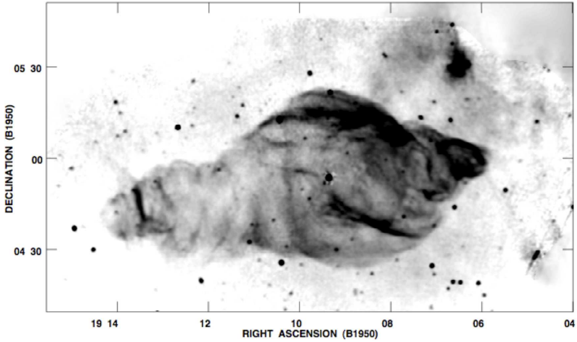
Figure 7–2: VLA radio continuum image of W50 at 1465 MHz. The bright point source at the center (RA: \sim 19\ 09 Dec: \sim +04\ 53 ) is the black hole, the regions where the jets interact with the ISM are visible in the east (RA: \sim 19\ 13 Dec: \sim +04\ 40 ) and in the west (RA: \sim 19\ 07 Dec: \sim +05\ 00 ). Figure taken from [43].
