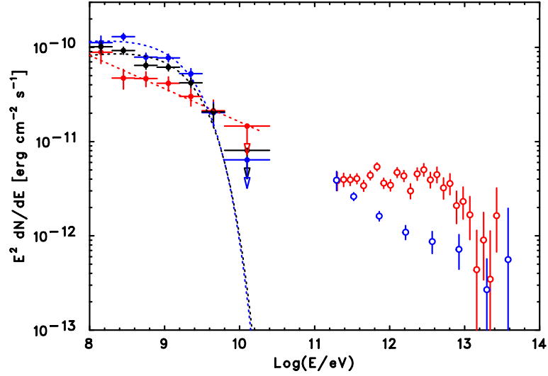
Figure 6–8: Fitted spectrum of LS 5039. Fermi data points are from likelihood fits in each energy bin. The black points (dotted line) represent the phase-averaged Fermi /LAT spectrum. The red data points (dotted line) represent the spectrum (overall fit) at inferior conjunction (Phase 0.45–0.9); blue data points (dotted line) represent the spectrum (overall fit) at superior conjunction (Phases, <0.45 and >0.9). Data points above 100 GeV are taken from H.E.S.S observations [13]; the data from H.E.S.S are not contemporaneous with Fermi , though they do cover multiple orbital periods. Figure taken from [1].
