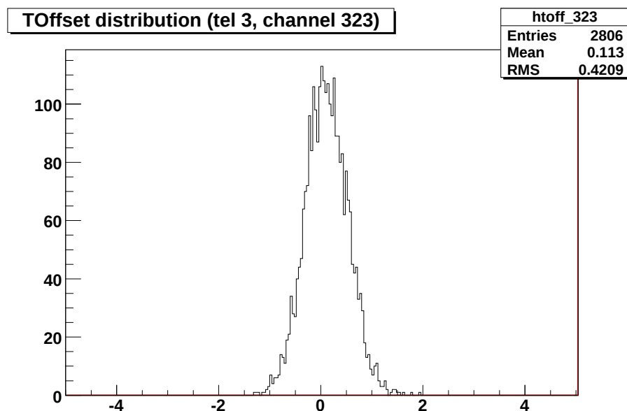
Figure 4–3: Example of a T_{zero} distribution for a single pixel over one laser run. The horizontal scale is in FADC samples (of 2 ns).
