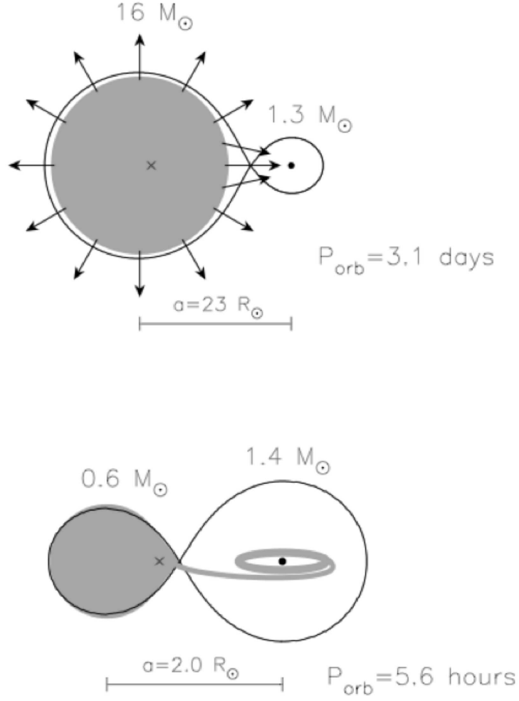
Figure 6-2: Top: Illustration of accretion through stellar wind. The neutron star is fed by a strong high-velocity stellar wind. Bottom: Illustration of the Roche lobe overflow. The neutron star is surrounded by an accretion disk which is fed by Roche-lobe overflow. Figure taken from [156].
