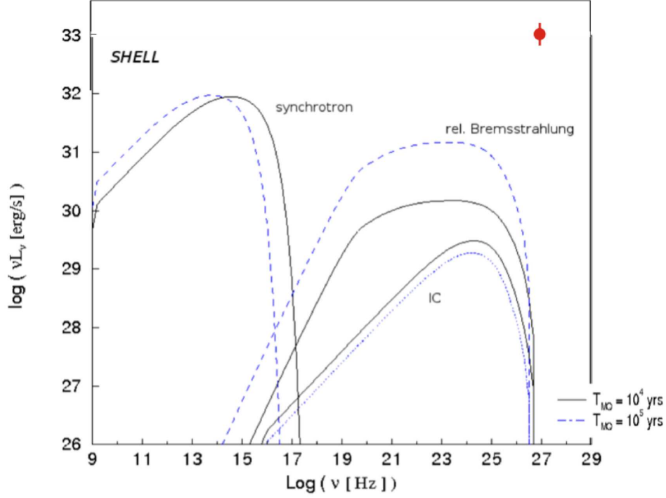
Figure 7–17: SED obtained in the Bordas model in the shell region using Q_{jet} = 10^{37} \text{ erg s}^{-1} and n_{ISM} = 1 \text{ cm}^{-3} . The VERITAS flux point (in red) has been added to the plot. Figure adapted from [23].
