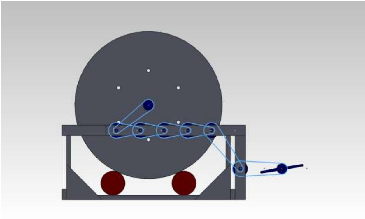
Figure 16- Front view of the assembly of the bicycle-powered composter.
