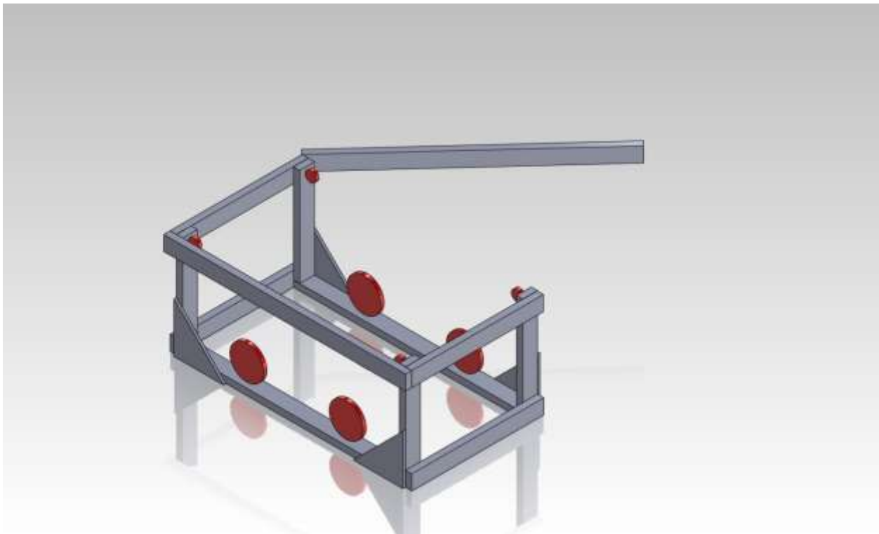
Figure 14- Isometric view of the frame (open) of the bicycle-powered composter.
