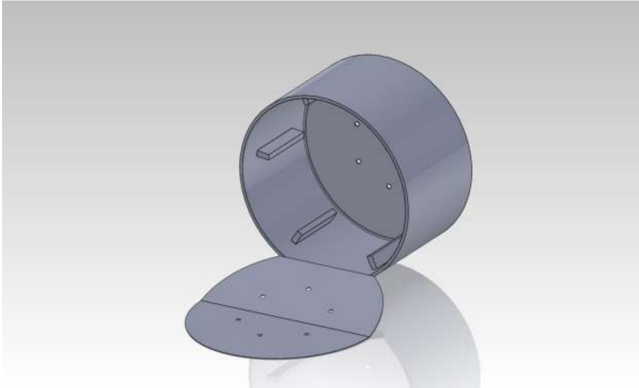
Figure 7- Isometric view of the unloading position of the cylindrical drum of the bicycle-powered composter.
