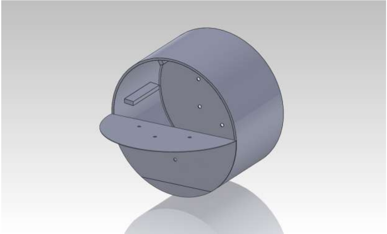
Figure 6- Isometric view of the loading position of the cylindrical drum of the bicycle-powered composter.
