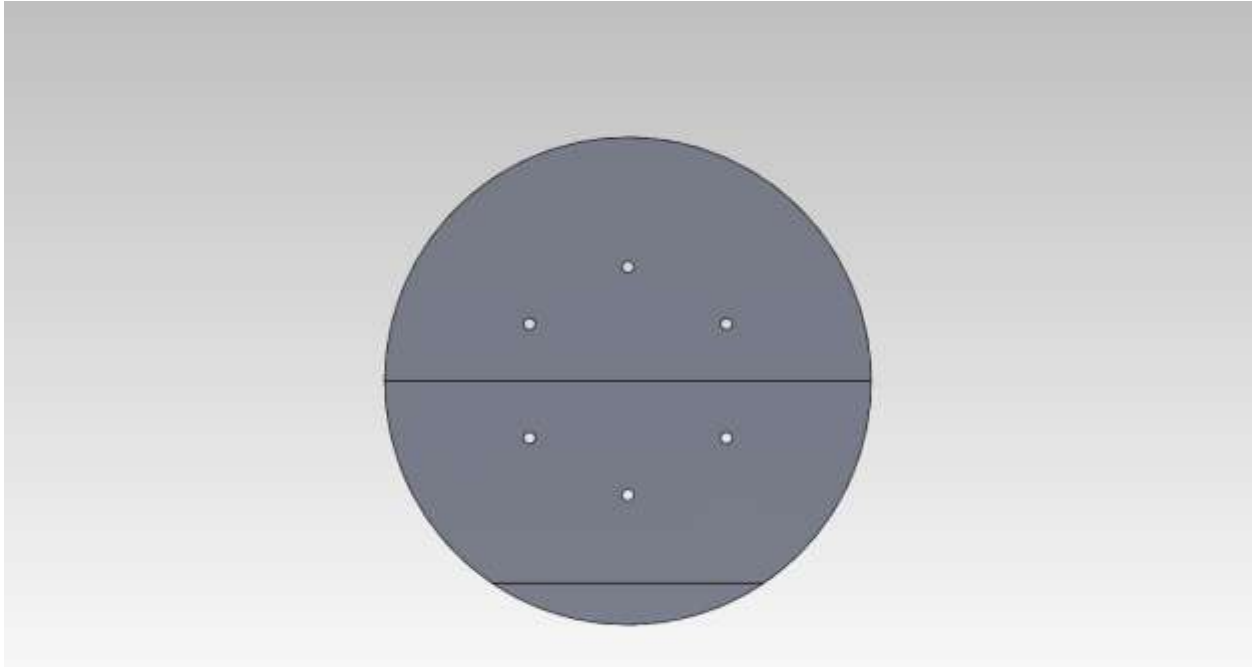
Figure 5- Rear view of the cylindrical drum of the bicycle-powered composter.
