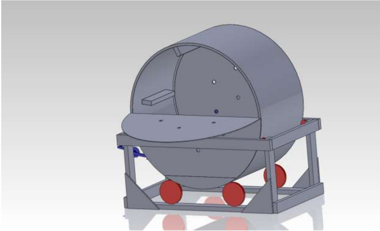
Figure 18- Isometric view of the loading position of the assembly of the bicycle-powered composter.
