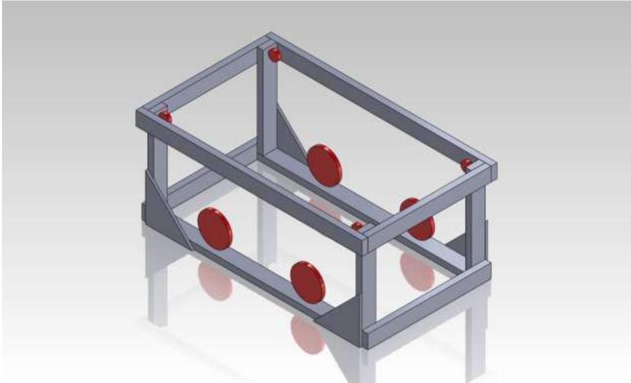
Figure 13- Isometric view of the frame (closed) of the bicycle-powered composter.
