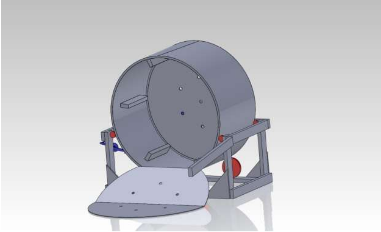
Figure 19- Isometric view of the unloading position of the assembly of the bicycle-powered composter.
