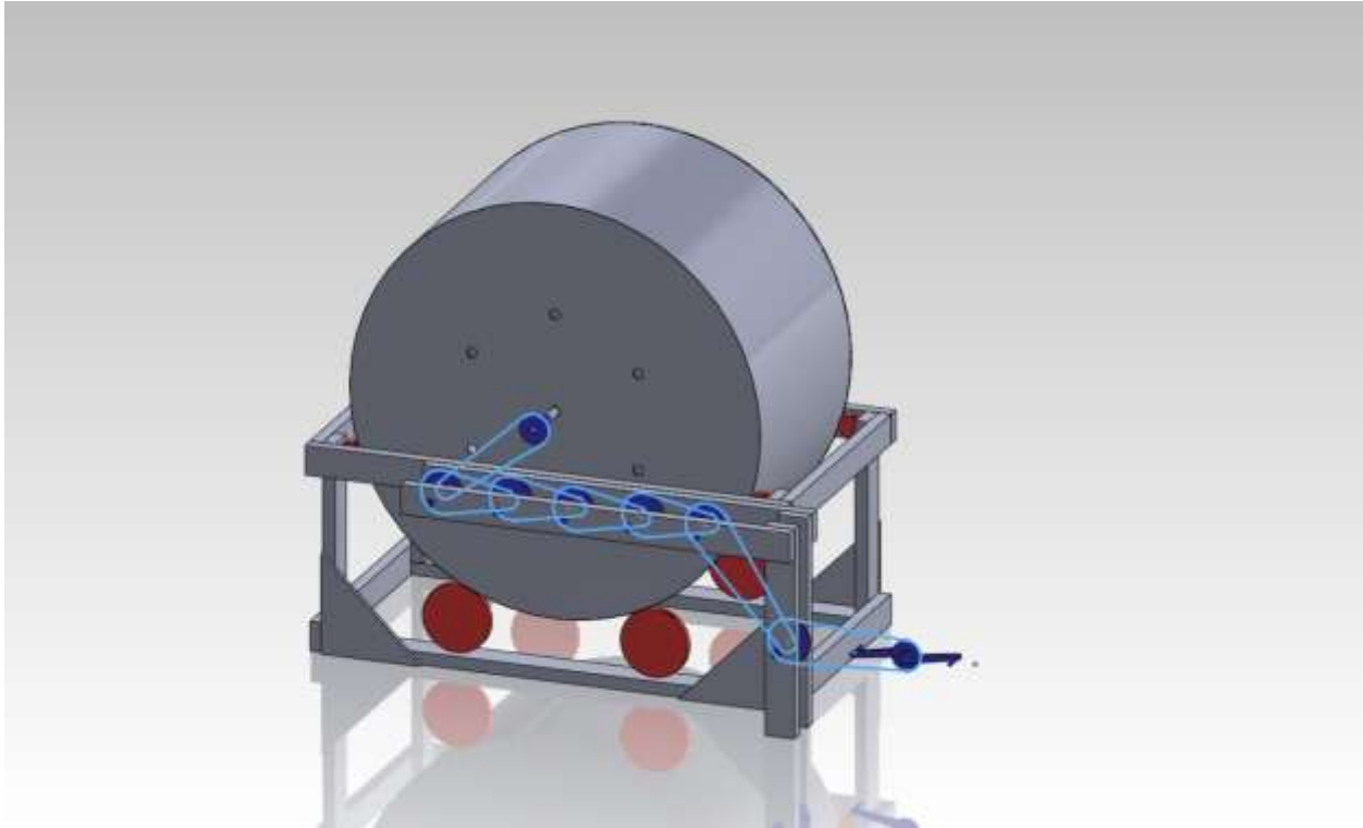
Figure 15- Dimetric view of the assembly of the bicycle powered composter.
