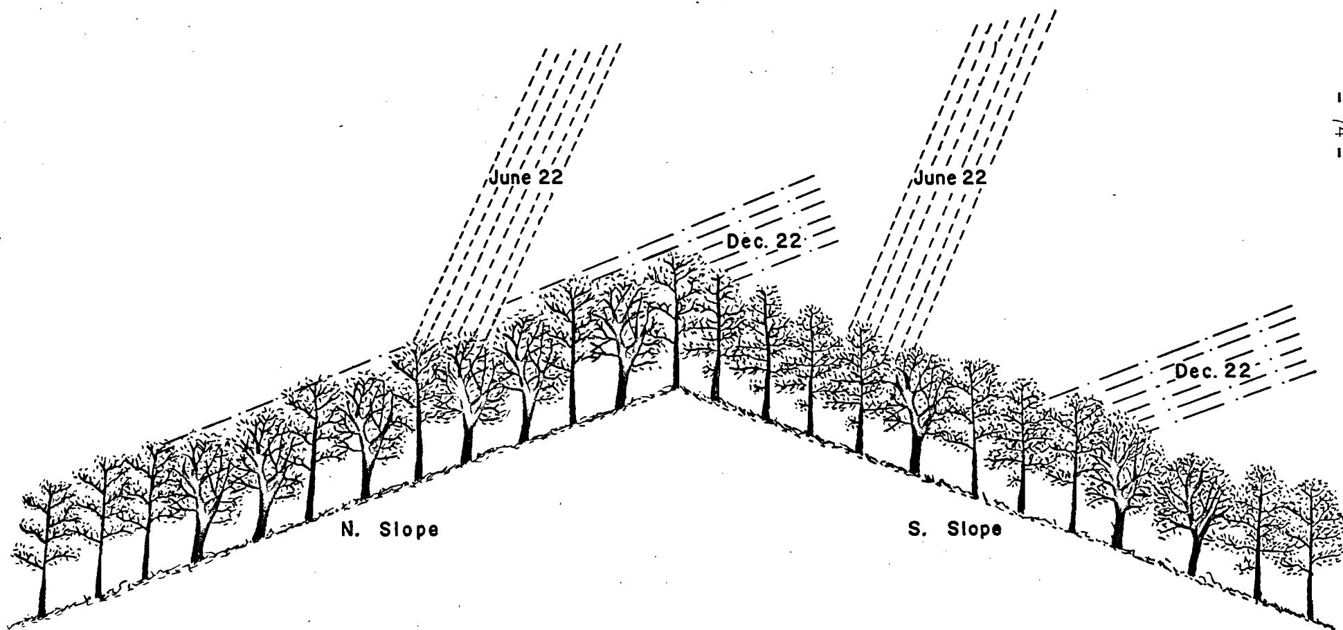
FIGURE 6. The influence of forest cover on the intensity of solar radiation for south and north hillsides of 20^\circ slope. Solar radiation is shown for the noon hour period during summer and winter solstices.
