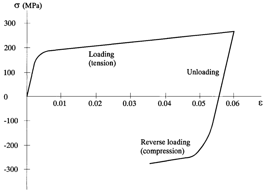
Fig. (2.20) Stress–strain curve for uniaxial tensile loading and unloading, followed by compression for Al 6022-T4 alloy (adapted from Cleveland and Ghosh, 2002)
