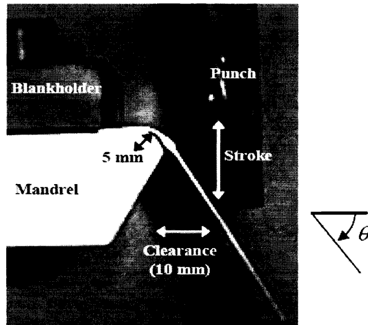
Fig. (2.35) Bending experiment setup
