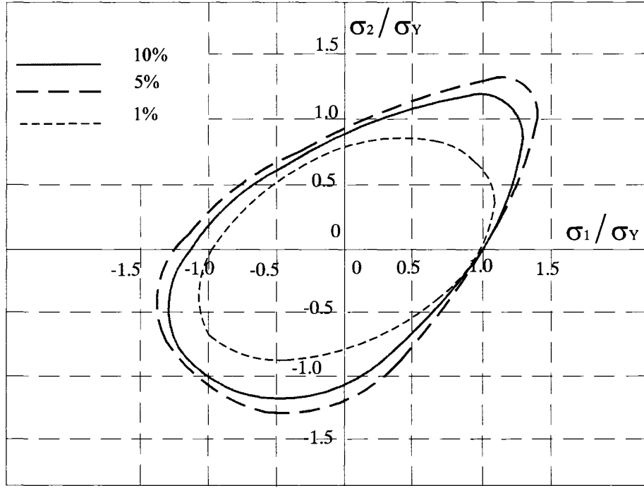
Fig. (2.12) Yield loci for Mg-4%Li alloy at different strain levels (adapted from Cazacu et al. , 2004)
