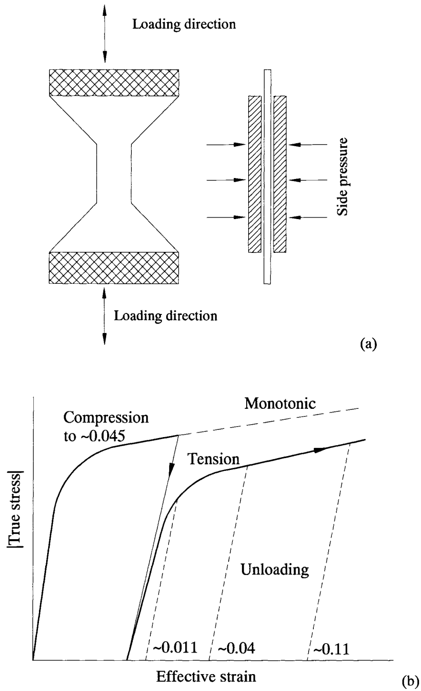
Fig. (2.25) Schematic of compression/tension/unloading test: (a) specimen geometry and the anti-buckling fixture, and (b) general load path (adapted from Wang et al. , 2004b)
