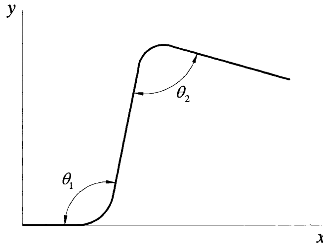
Fig. (2.41) Definition of springback angles according to Park and Oh (2004)
