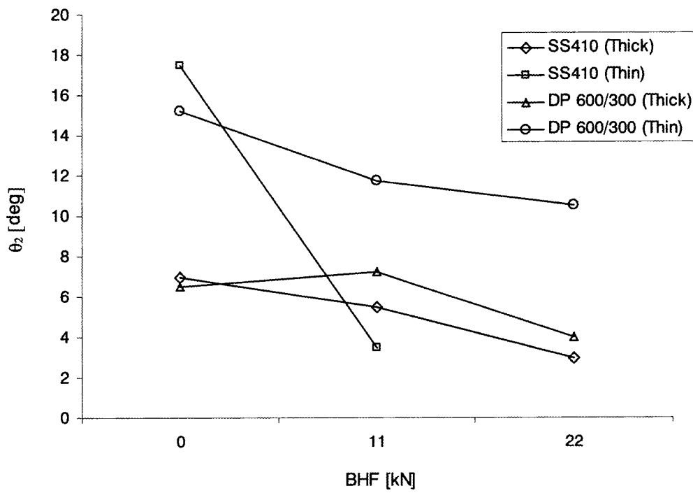
Fig. (4.32) Effect of BHF on springback angles for thick and thin steel specimens, (a) \theta_1 and (b) \theta_2
