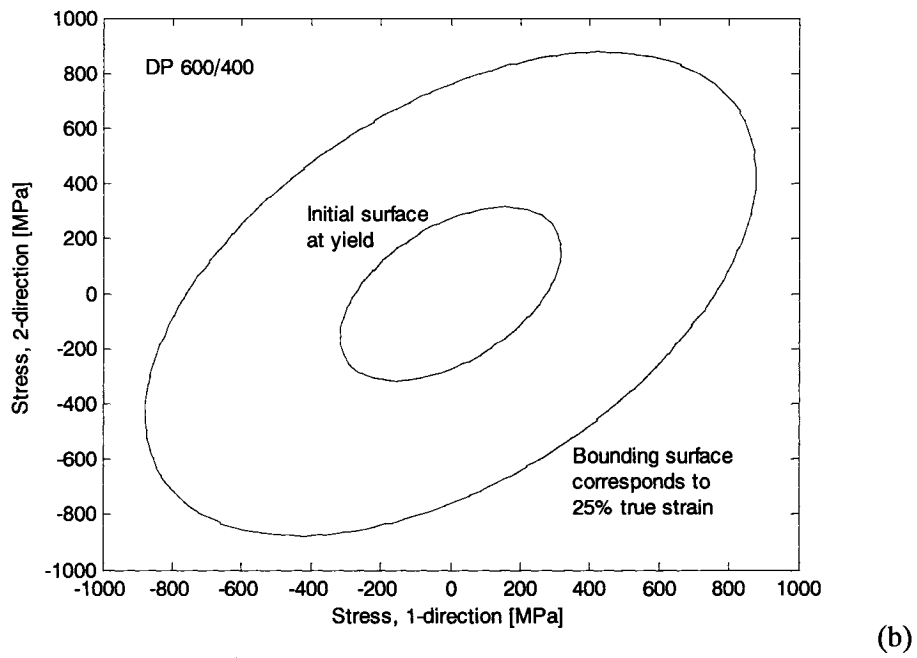
Fig. (5.10) Initial and bounding yield surfaces for (a) thick and thin DP600/300, and (b) DP600/400
