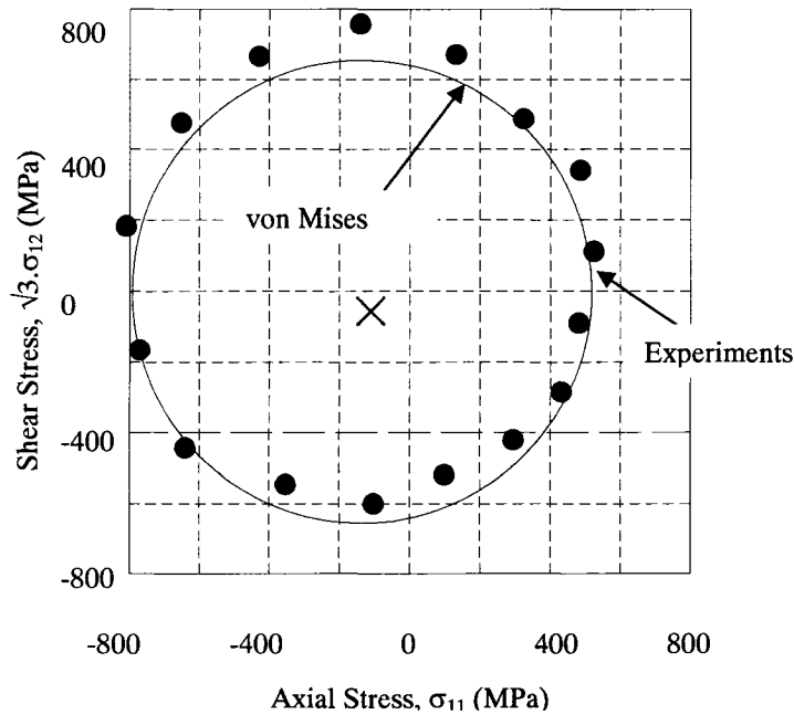
Fig. (2.27) Yield loci of aged inconel 718 at 25 °C compared to the von Mises yield surface (adapted from Gil et al. , 1999b)
