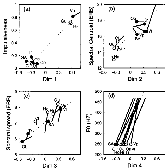
FIG. 7. Experiment IIb (11 semitones). Scatter plots relating each signal descriptor to the MDS dimension that it explains best. (a) Impulsiveness versus dimension 1. (b) Spectral centroid versus dimension 2. (c) Spectral spread versus dimension 3. (d) F_0 versus dimension 4. For each instrument, the symbol represents its position at note B3, and the opposite end of the line represents its position at note Bb4. Filled symbols indicate instruments for which the timbre changed significantly according to the analysis of C. Open symbols represent instruments for which it did not. Dotted lines represent regression lines.
